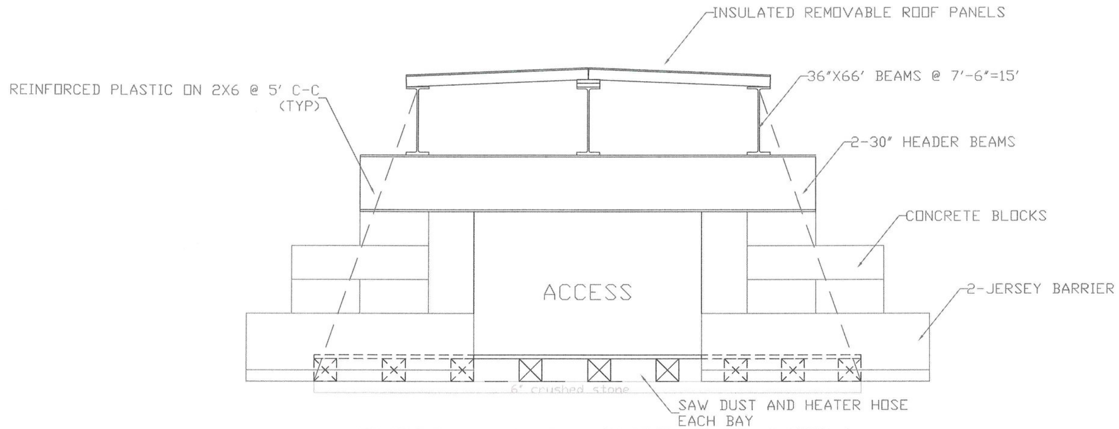
TYPICAL ENCLOSURE END VIEW
