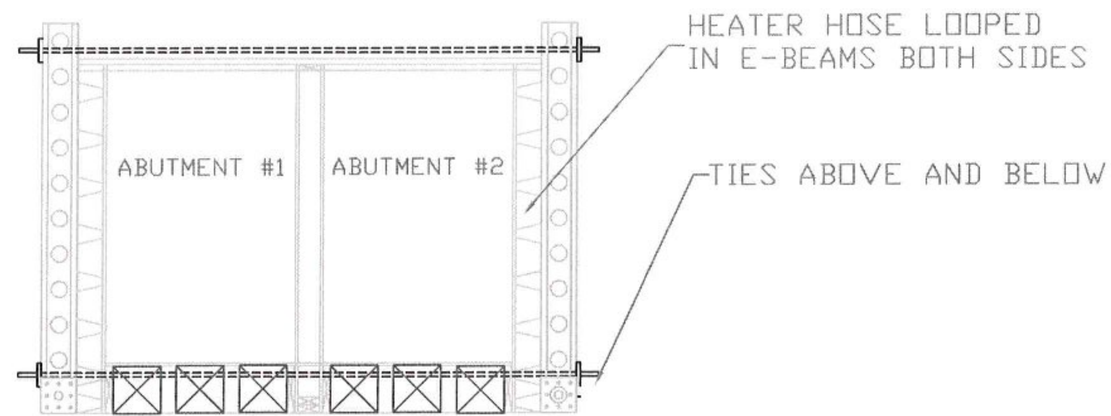
TYPICAL FORMING SECTION
