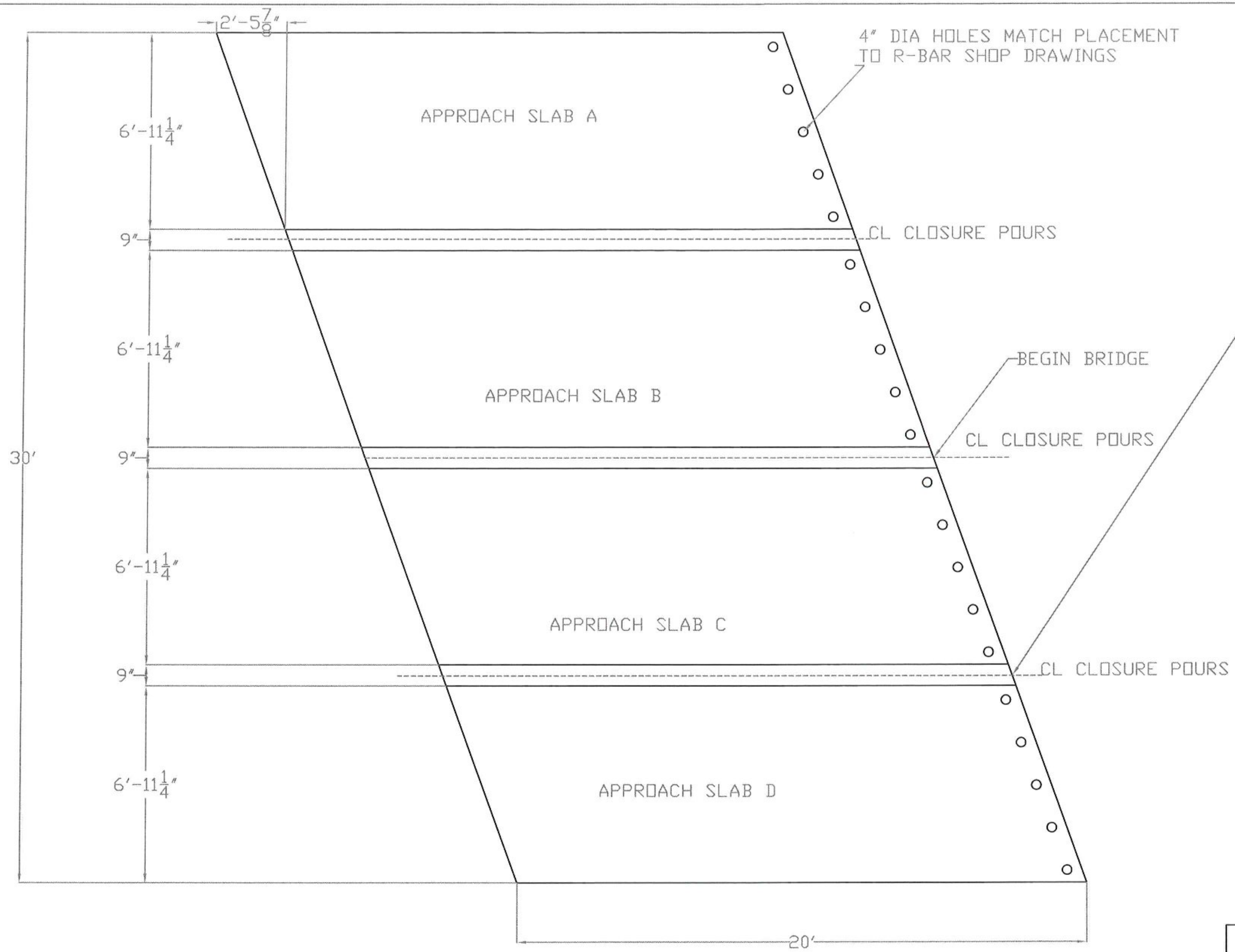
APPROACH SLAB 1 PLAN VIEW REVISION # 1 11-19-13 REVISION # 2 12-6-13
