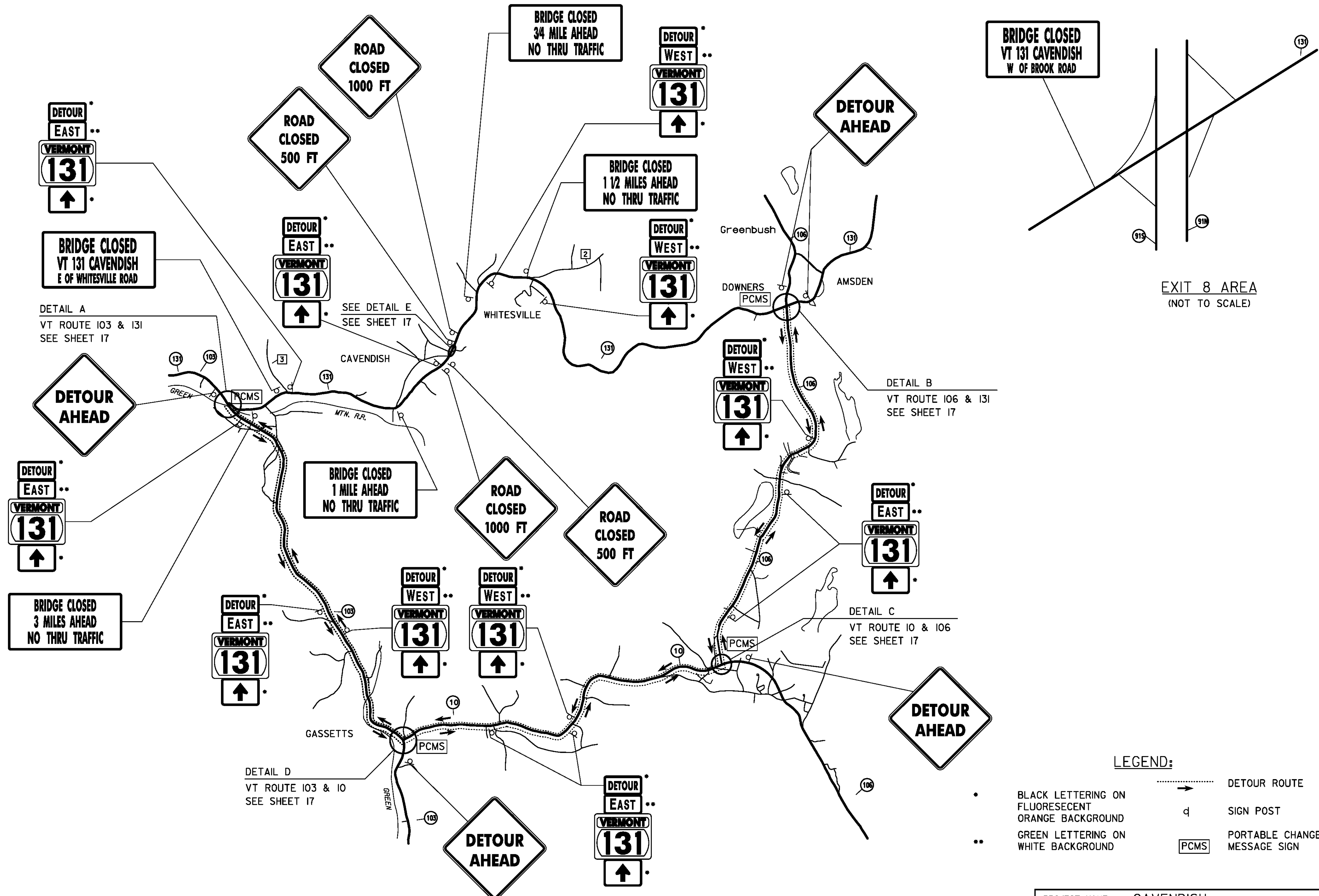
TRAFFIC DETOUR SIGNING PLAN (NOT TO SCALE)
