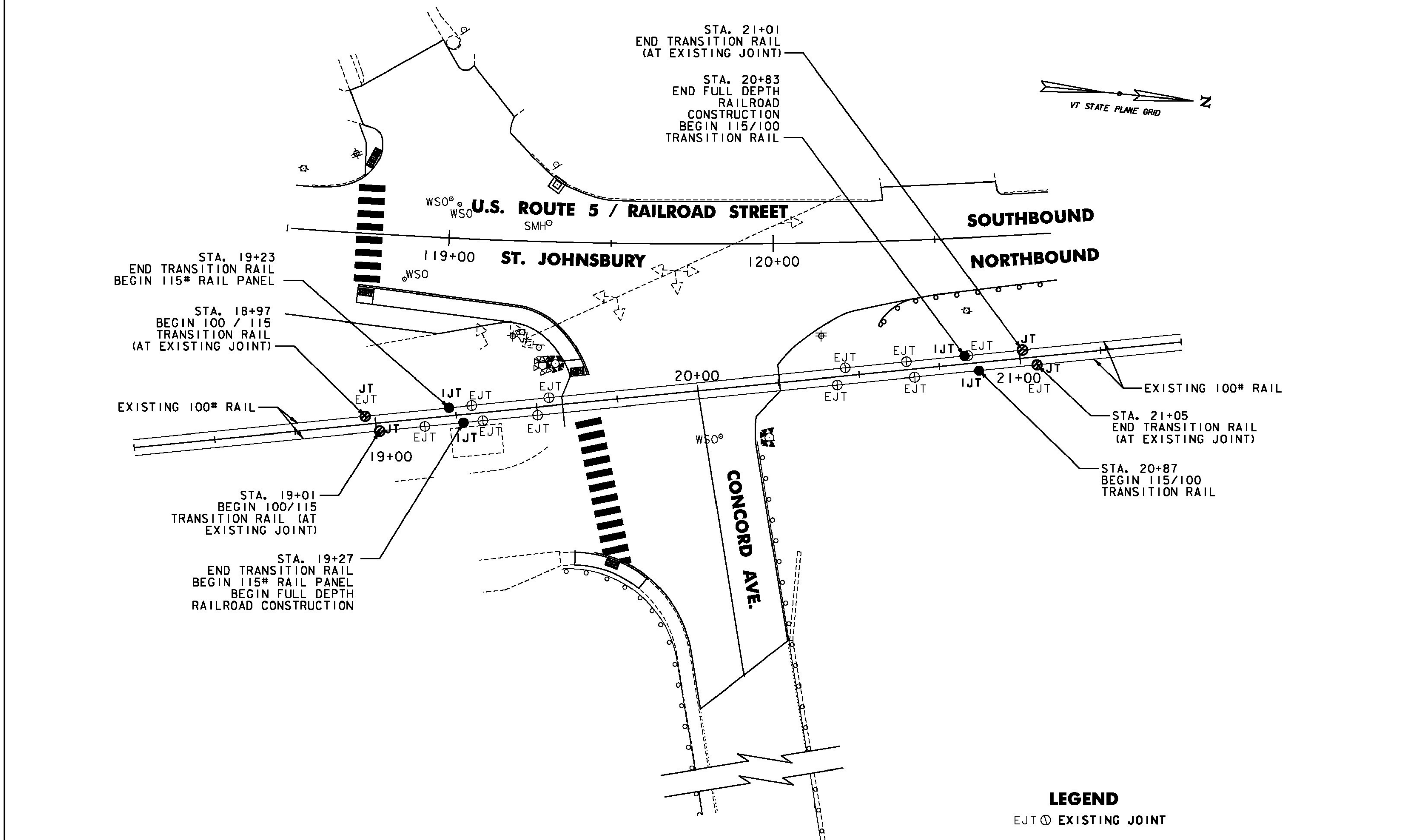
EXISTING AND PROPOSED RAIL JOINT LAYOUT CONCORD AVENUE AARDOT #850-938H
