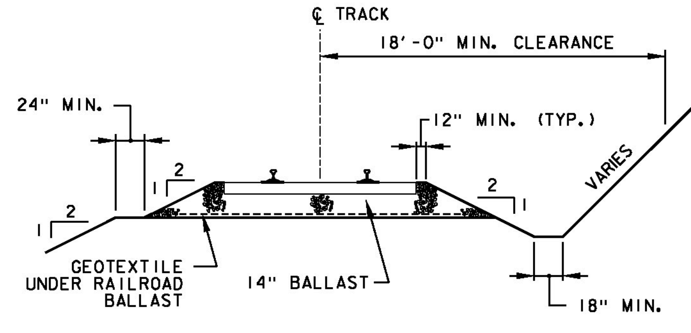
TYPICAL SECTION RAILROAD
