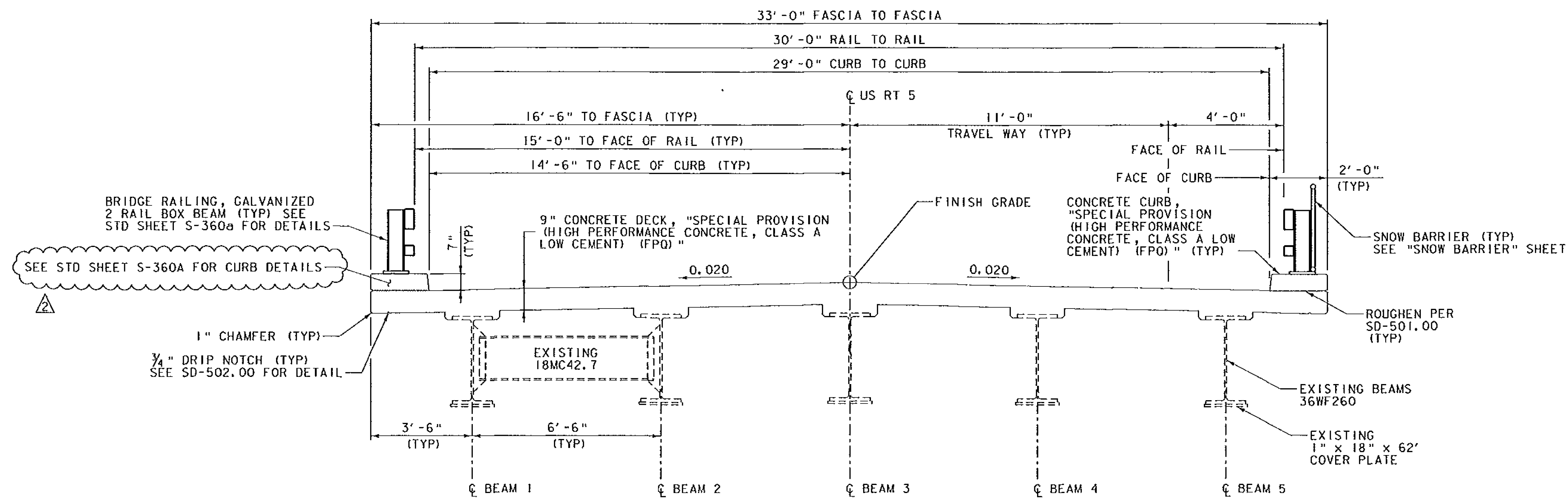
TYPICAL BRIDGE SECTION SCALE: 1/2" = 1'-0"
