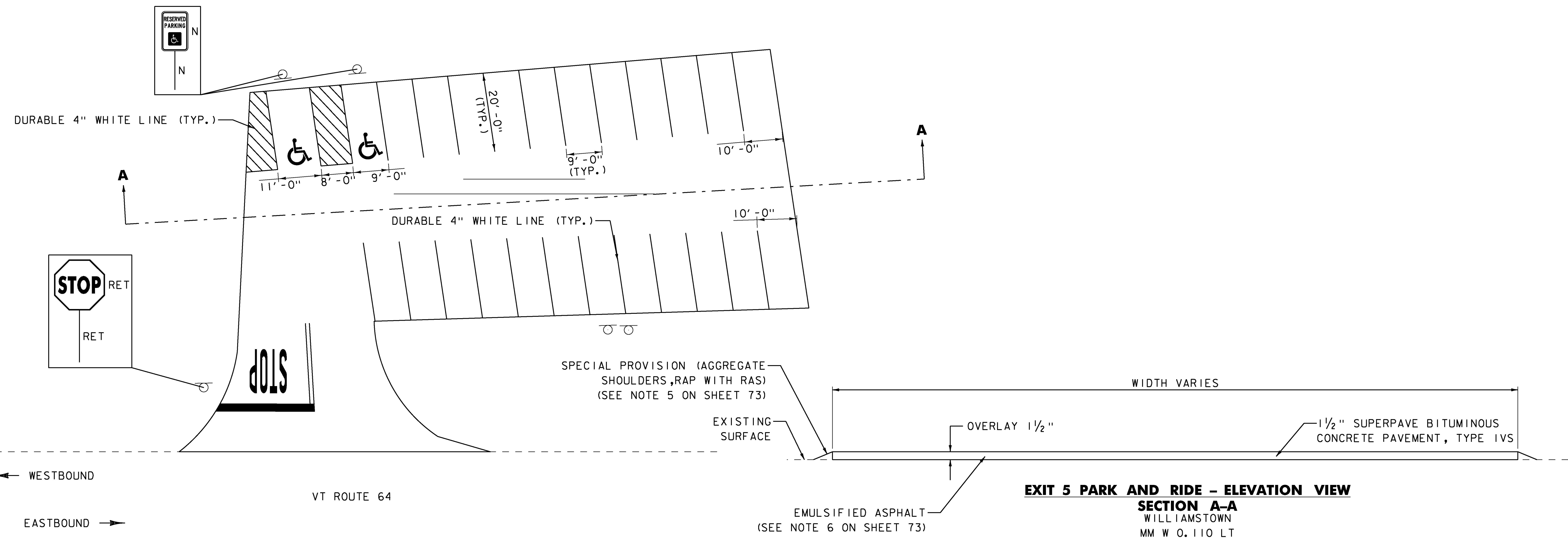
EXIT 5 PARK AND RIDE - PLAN VIEW
