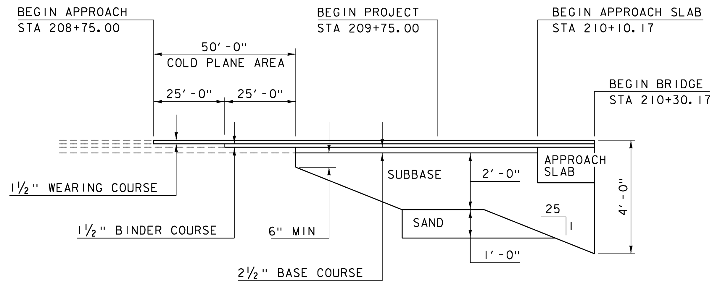
MATERIAL TRANSITION DIAGRAM I
