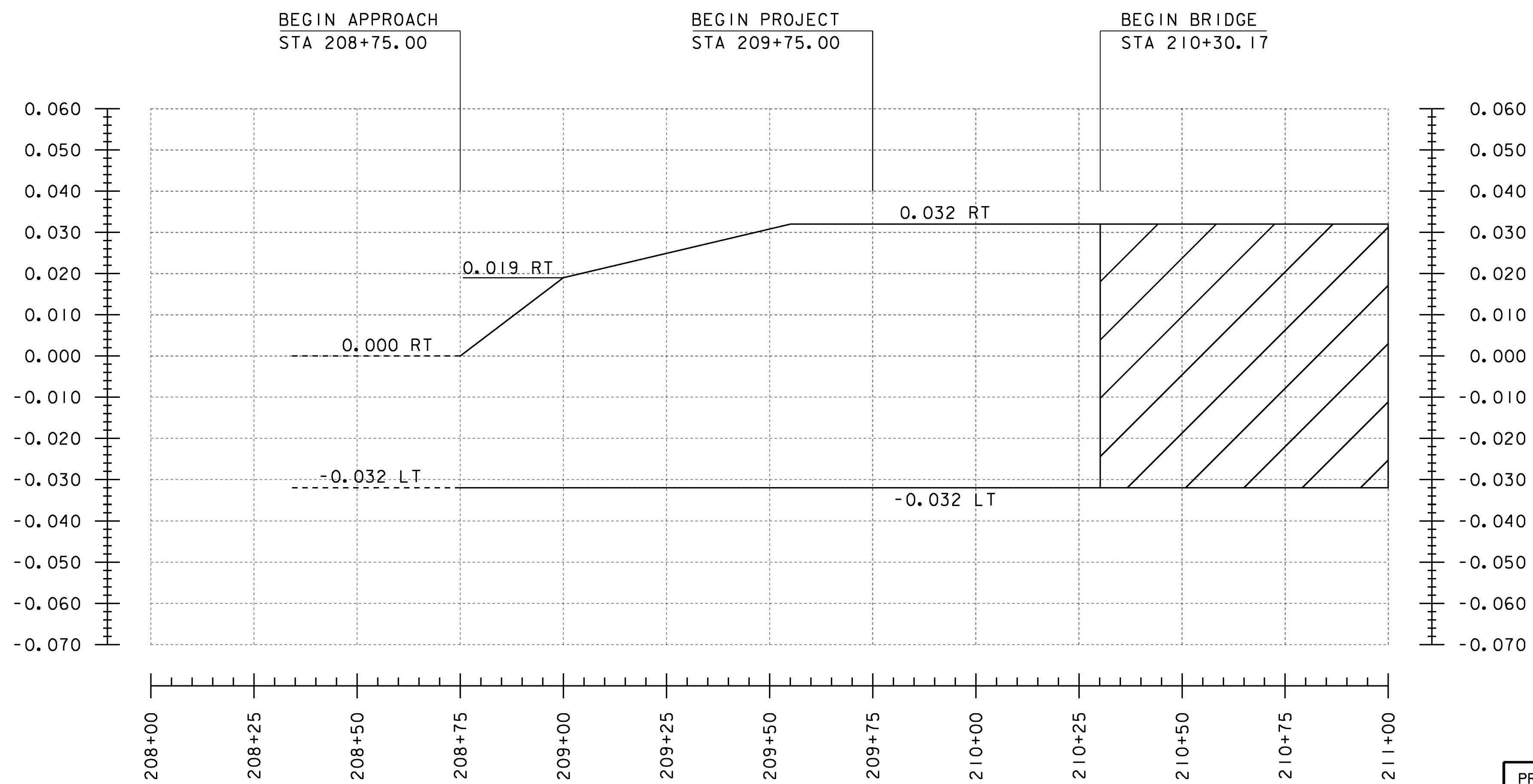
BANKING DIAGRAM I
