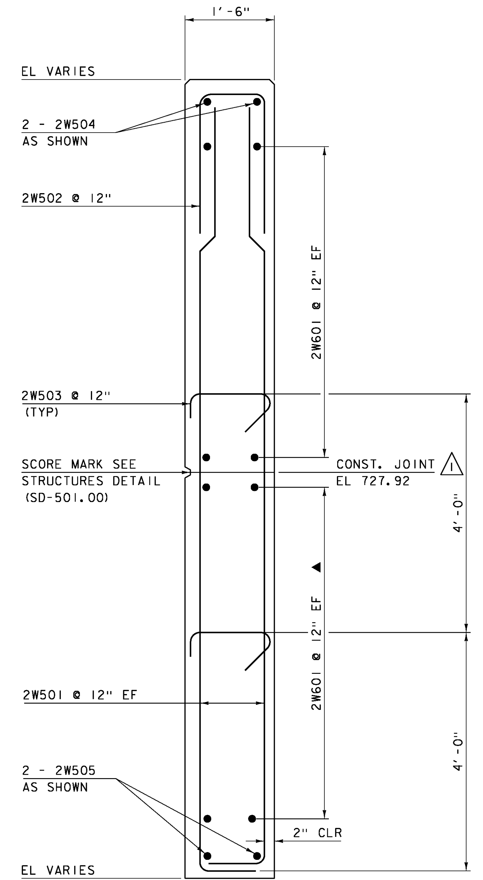
WINGWALL 2 TYPICAL SECTION SCALE 1"=1'-0"
