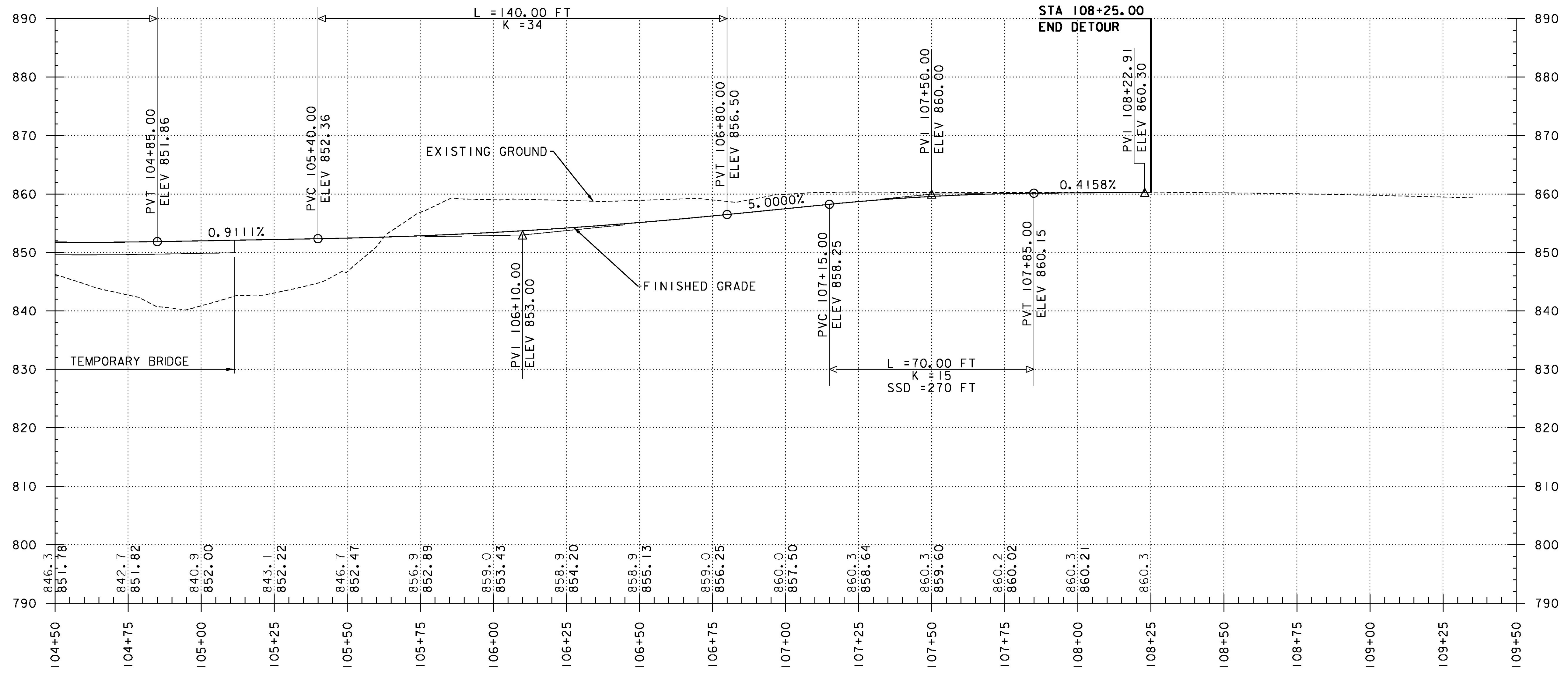
US 2 DETOUR PROFILE
