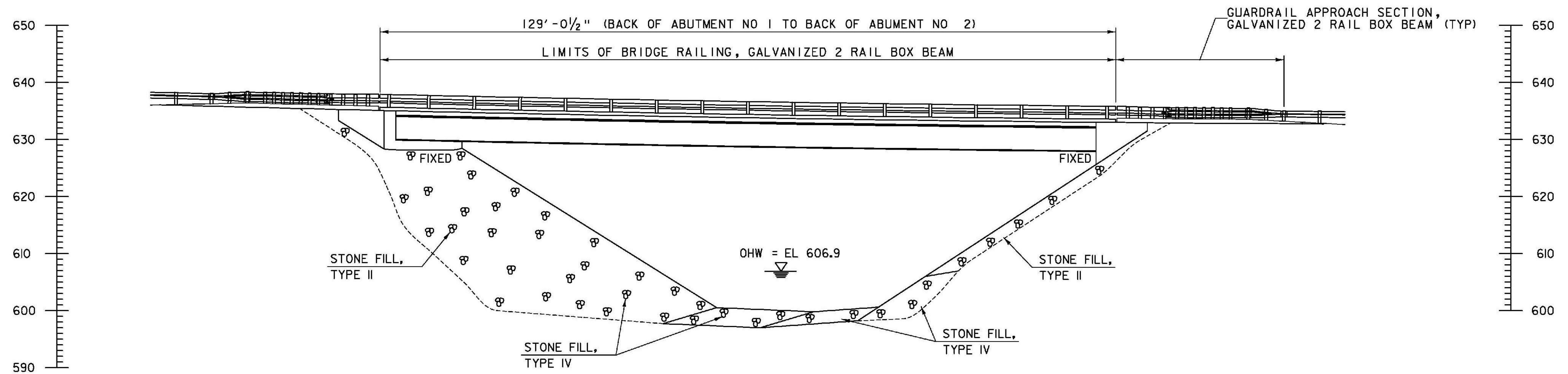
ELEVATION @ DOWNSTREAM FASCIA
