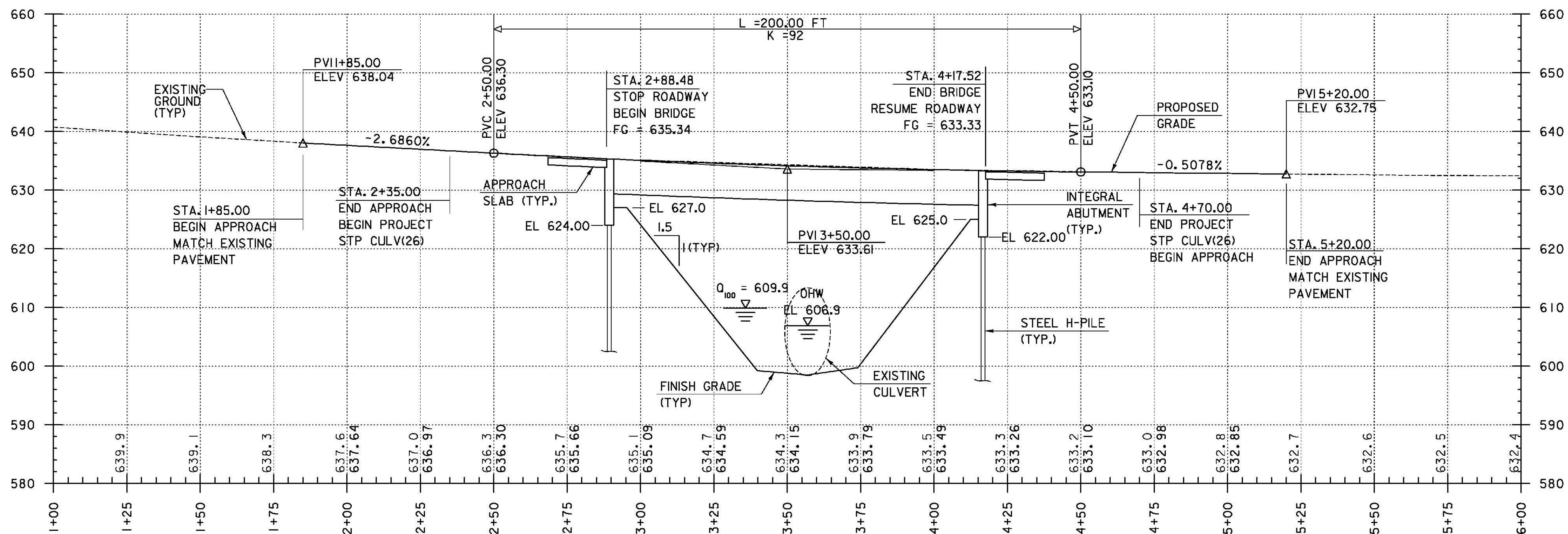
PROFILE - VT 15 STATIONING AND ELEVATIONS ARE IN FEET
