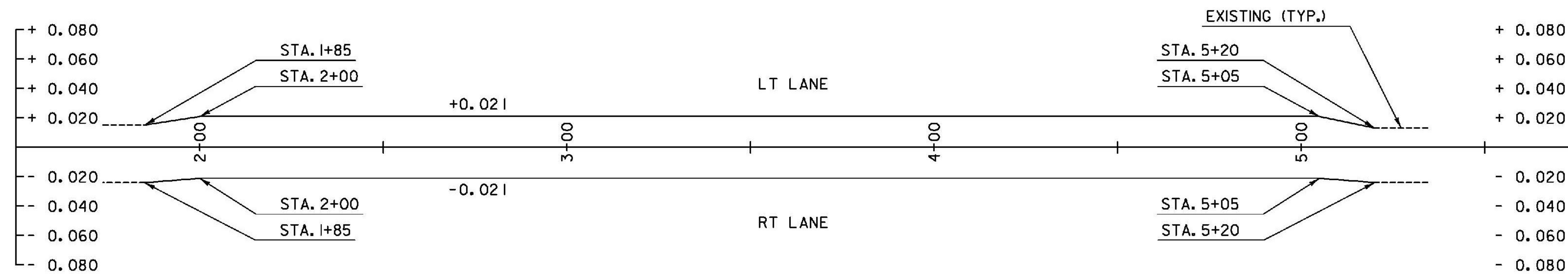
BANKING DIAGRAM STATIONS ARE IN FEET AND SUPERELEVATIONS ARE IN FT/FT
