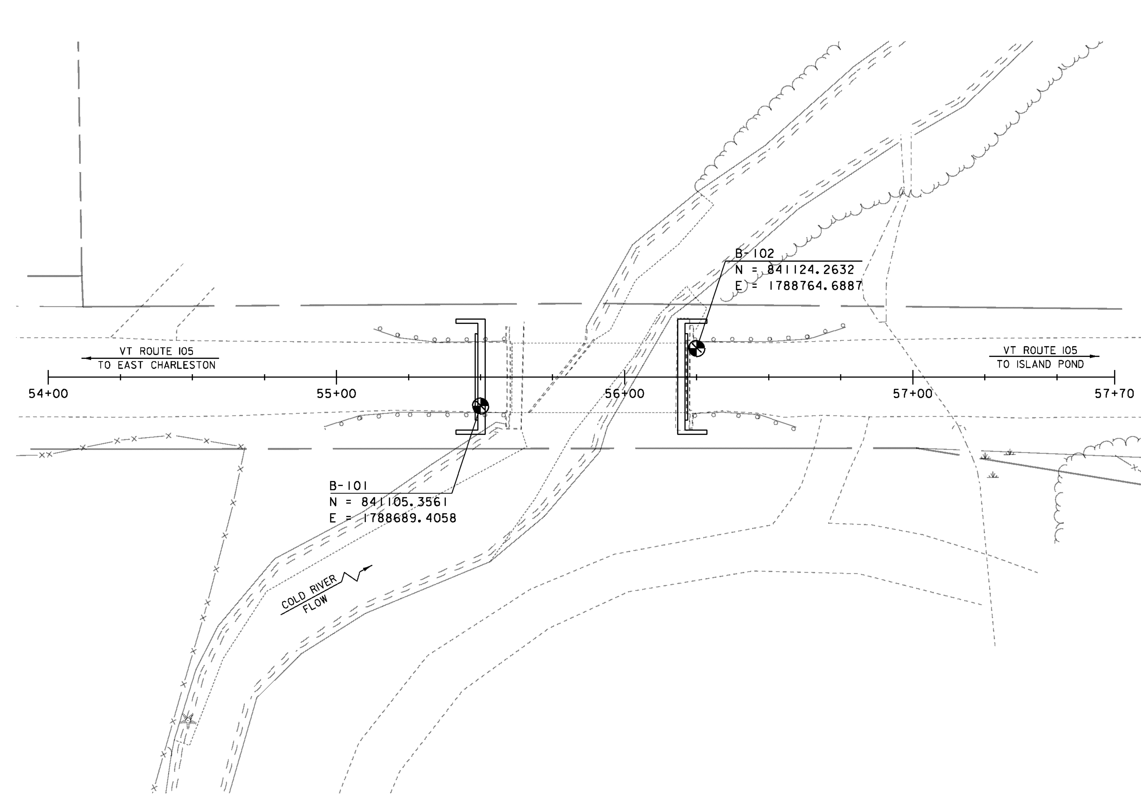
BORING LAYOUT SCALE 1" = 20'-0" 20 0 20
