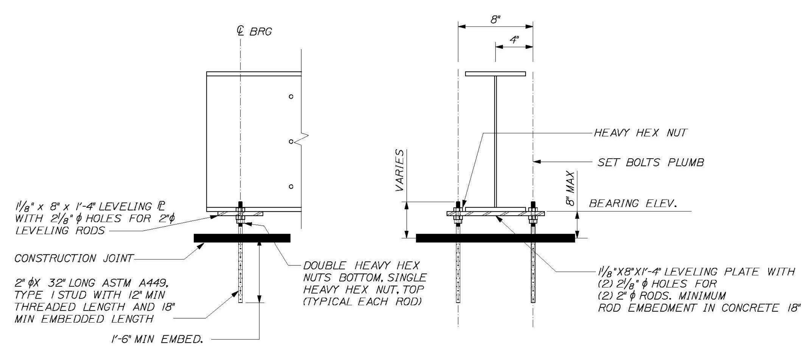
ANCHORAGE & BEARING DETAILS SCALE: 3/4" = 1'
