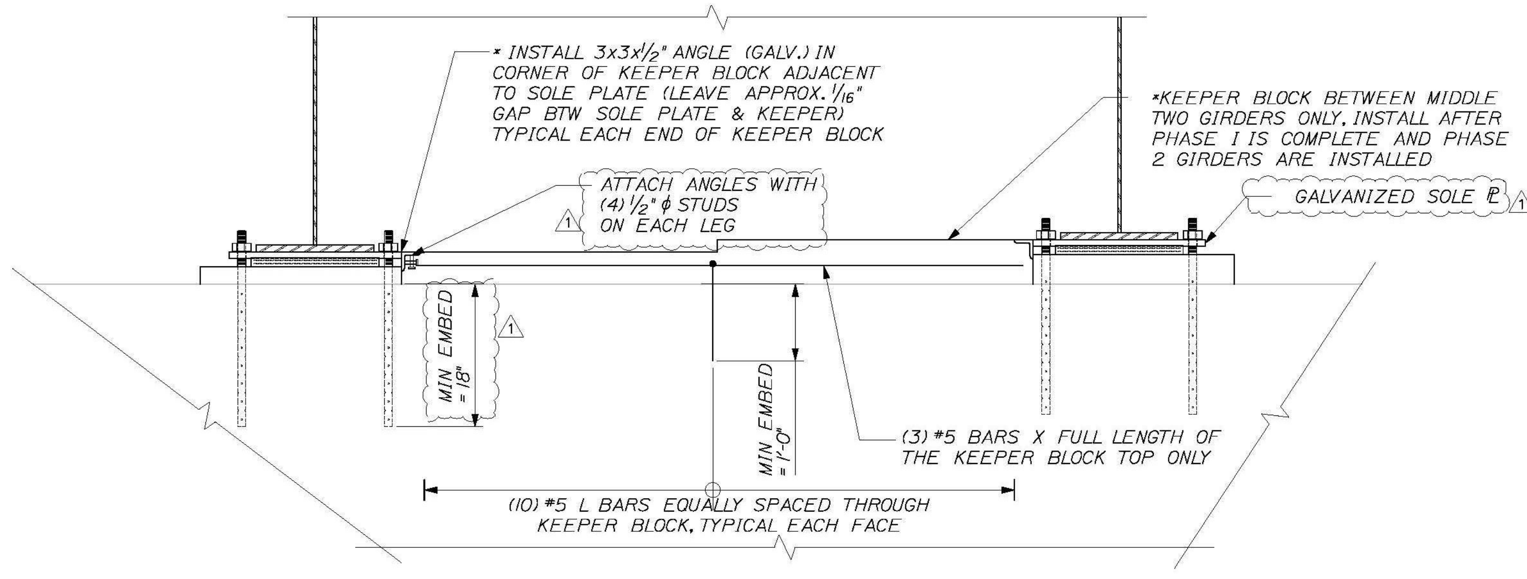
KEEPER BLOCK ELEVATION - INSTALL BETWEEN GIRDER LINES 2 & 3 AT EACH PIER SCALE: 3/4" = 1'
