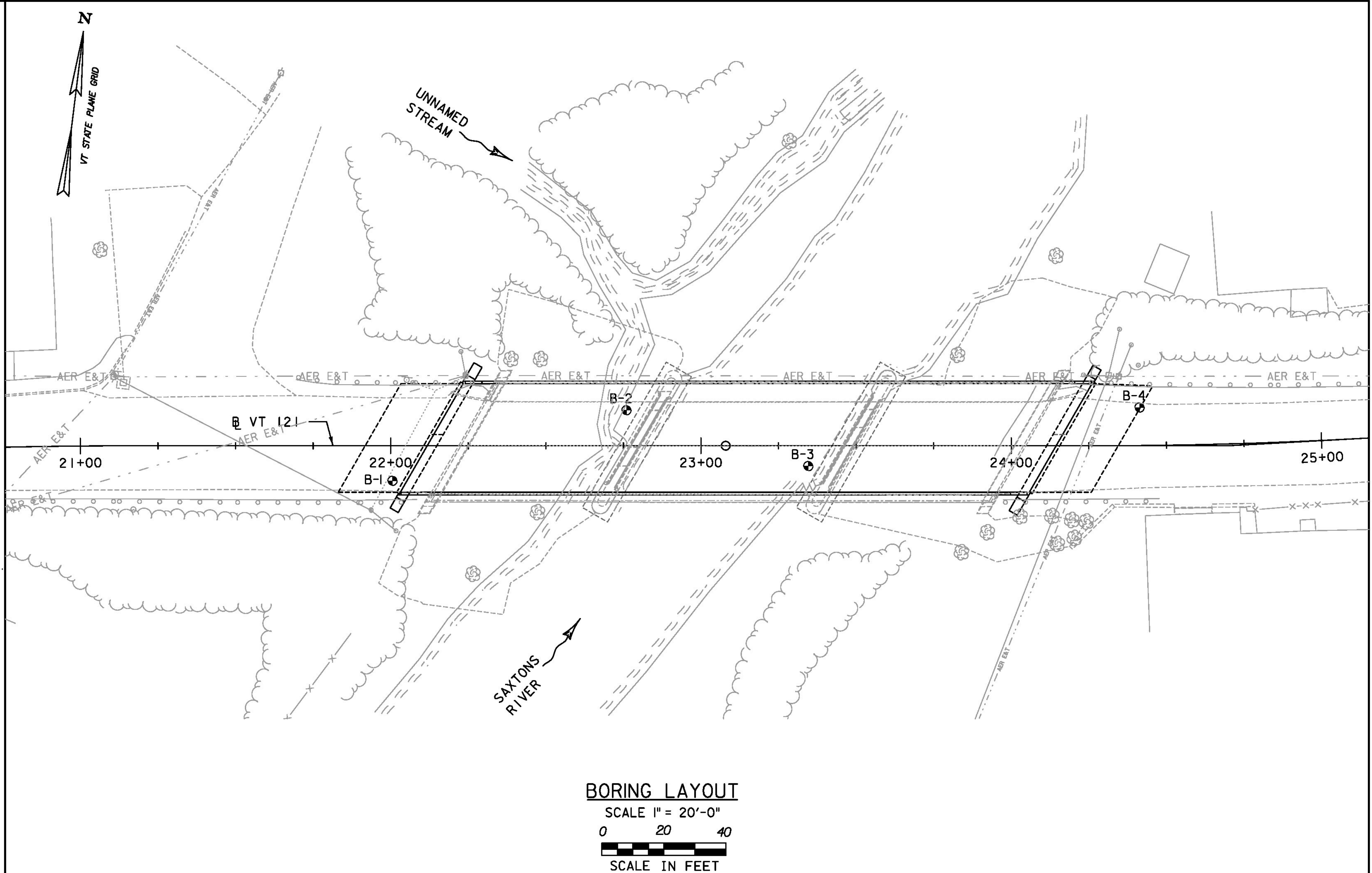
BORING LAYOUT
