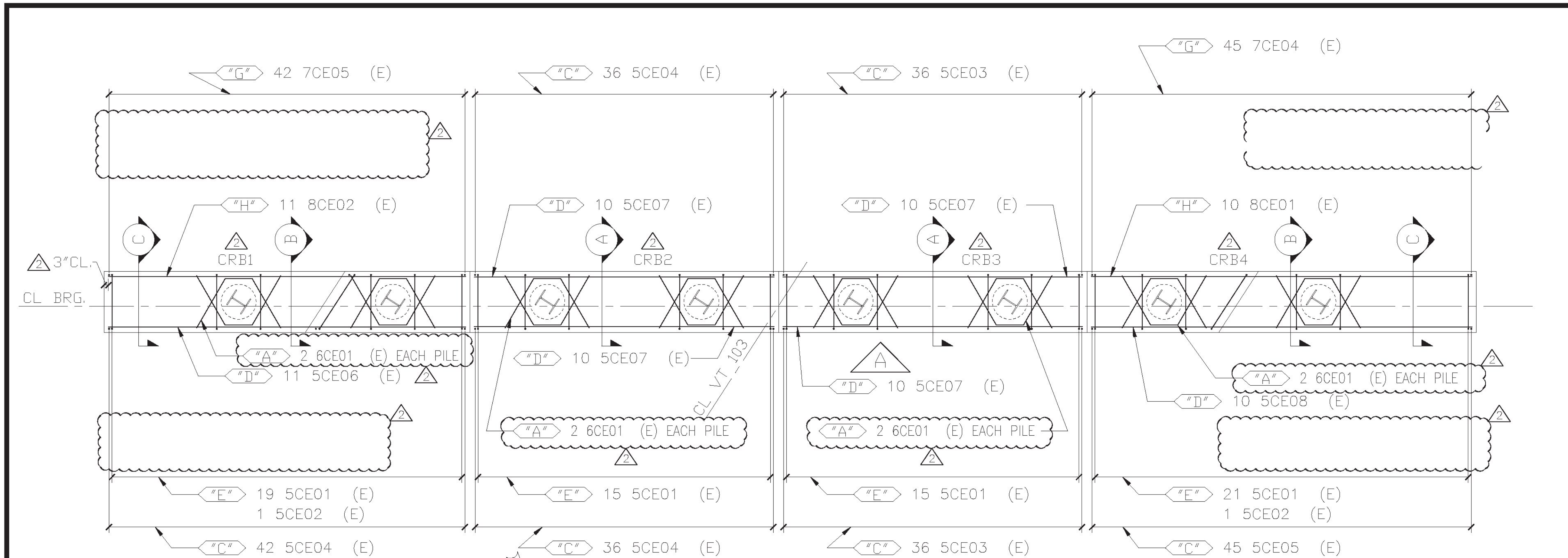
ABUTMENT NO. 1 PLAN CONTRACT DWG. REF. 42 OF 73 & 44 OF 73
