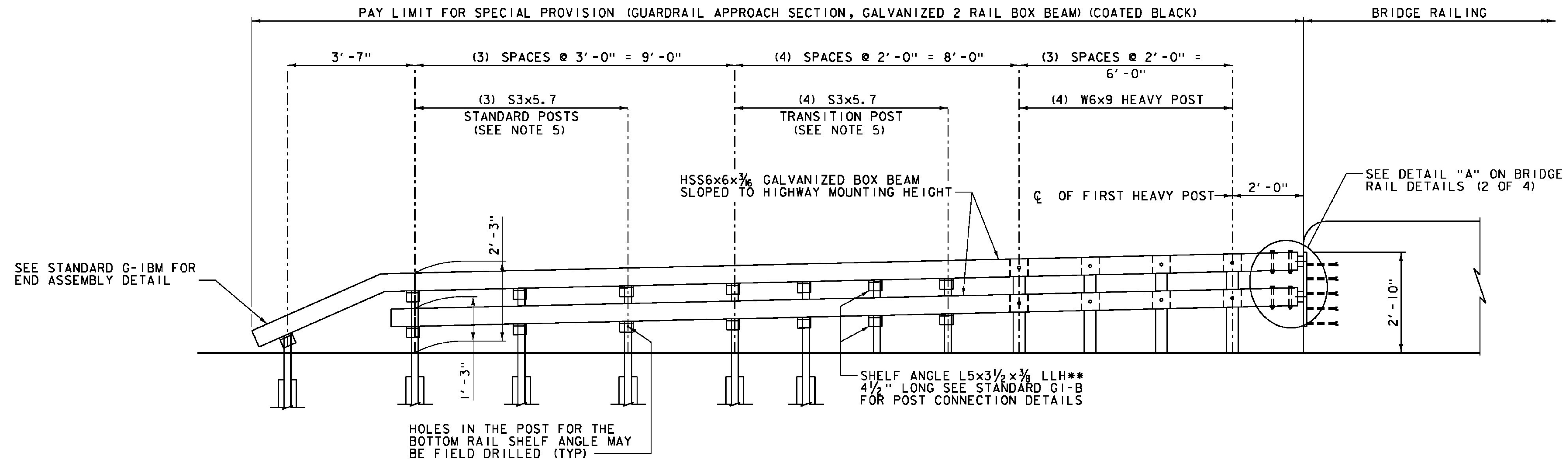
BOX BEAM APPROACH RAILING ELEVATION (NORTHWEST APPROACH) N. T. S.
