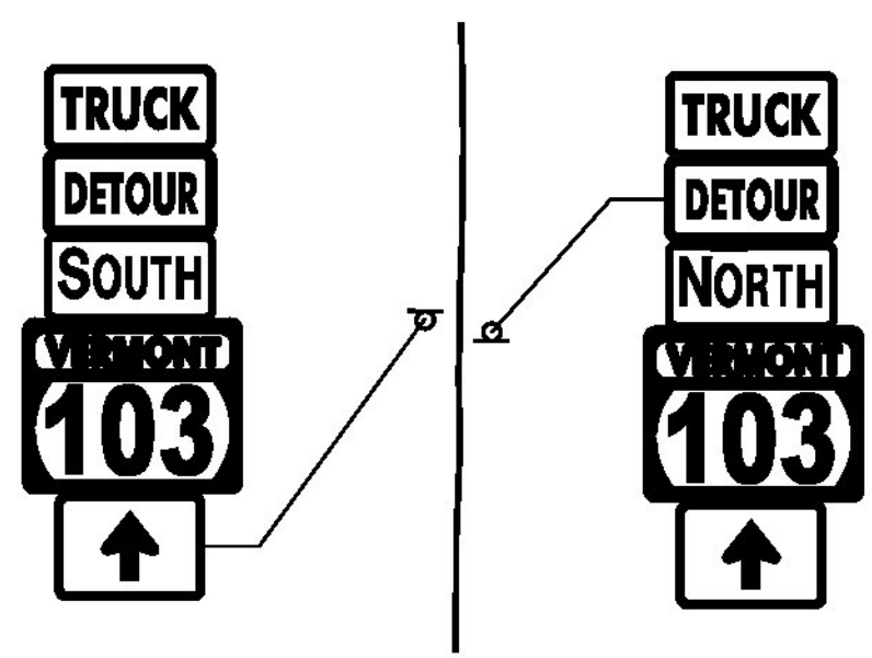
CONFIRMATORY ROUTE MARKER ASSEMBLY NOT TO SCALE
