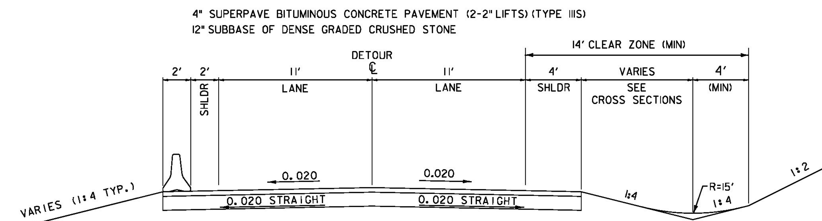
DETOUR TYPICAL SECTION STA 216+25.00 TO 221+97.54 NOT TO SCALE
