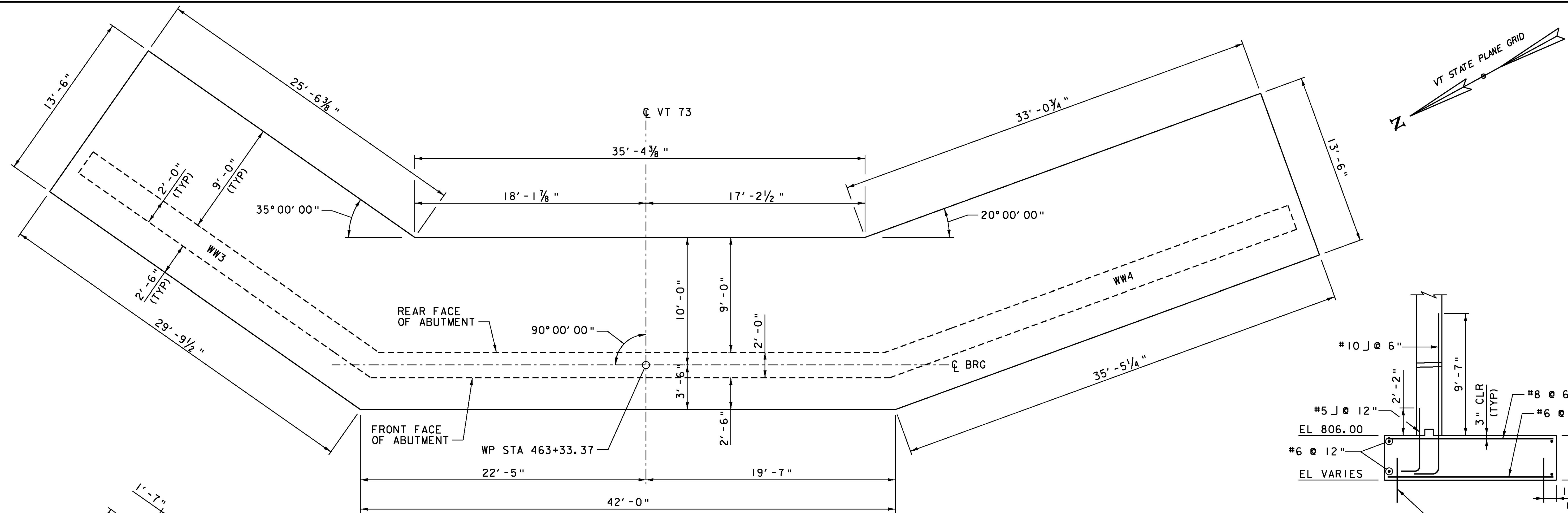
ABUTMENT NO 2 FOOTING MASONRY PLAN
