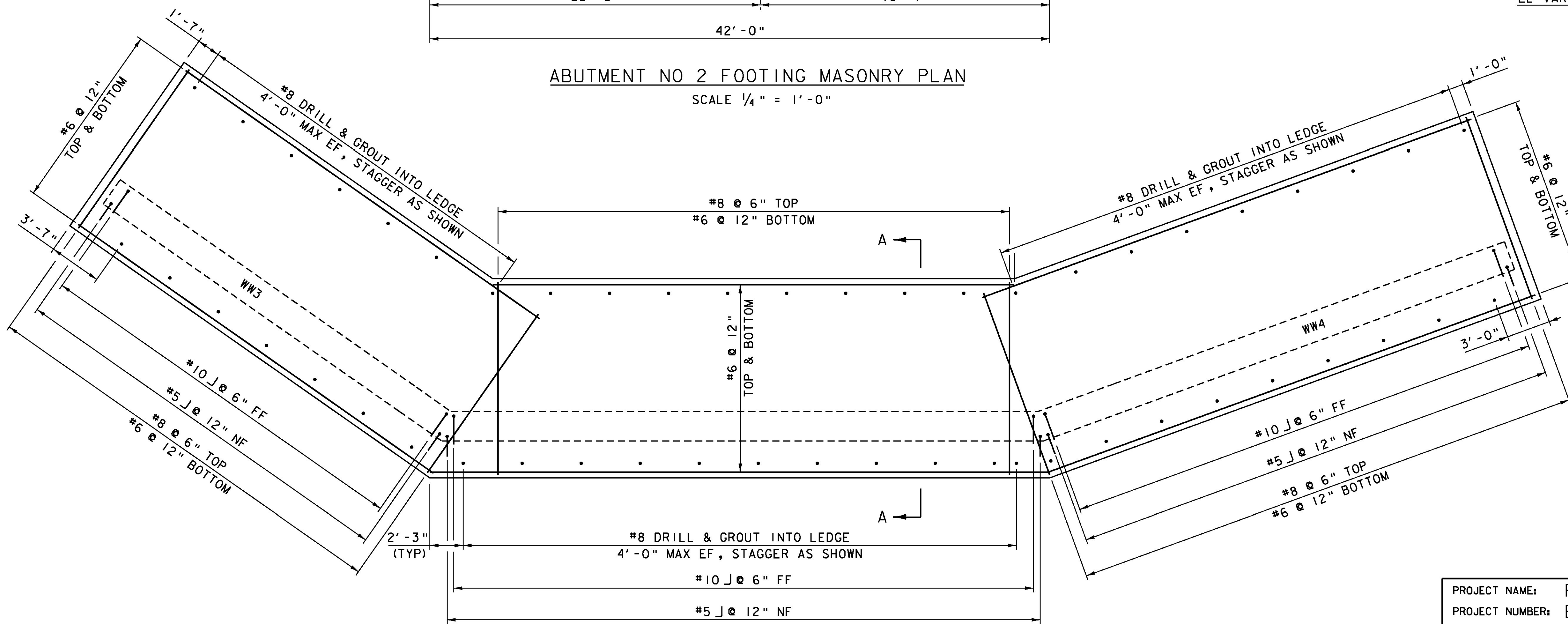
ABUTMENT NO 2 FOOTING REINFORCING PLAN
