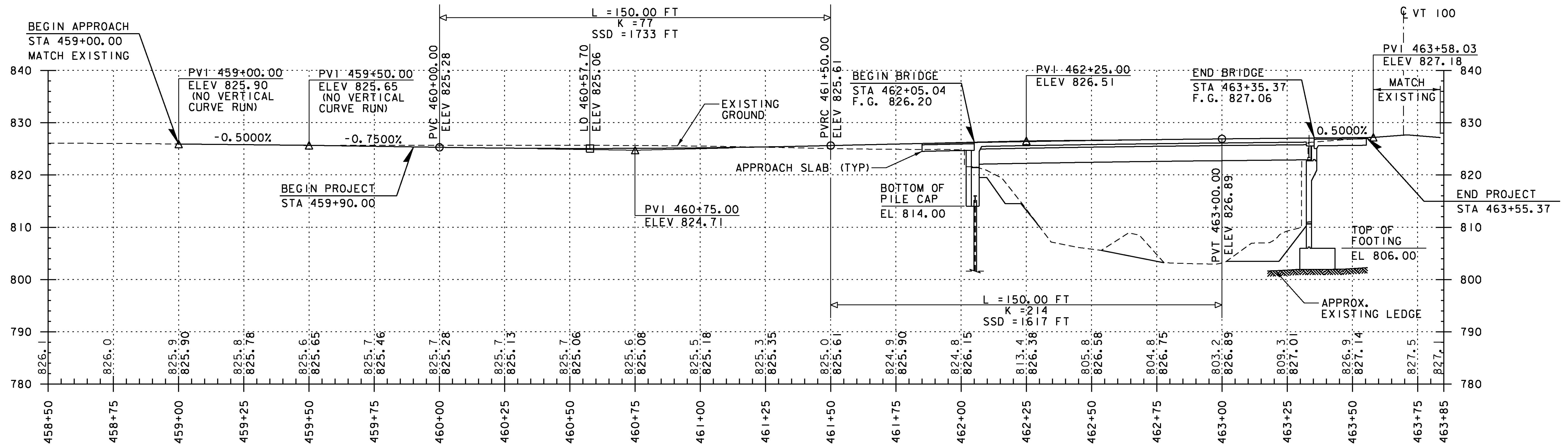
VT 73 PROFILE
