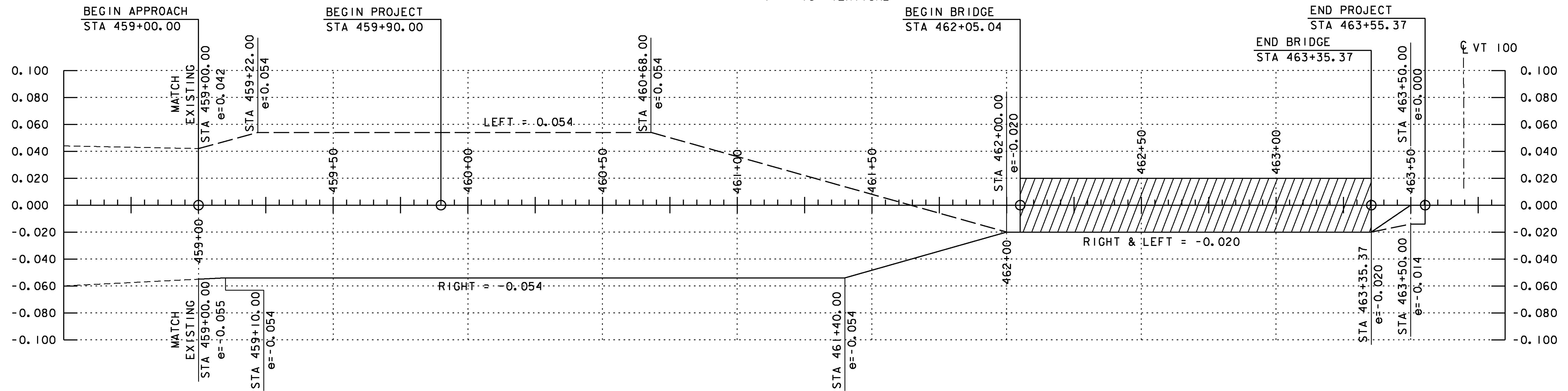
VT 73 BANKING DIAGRAM
