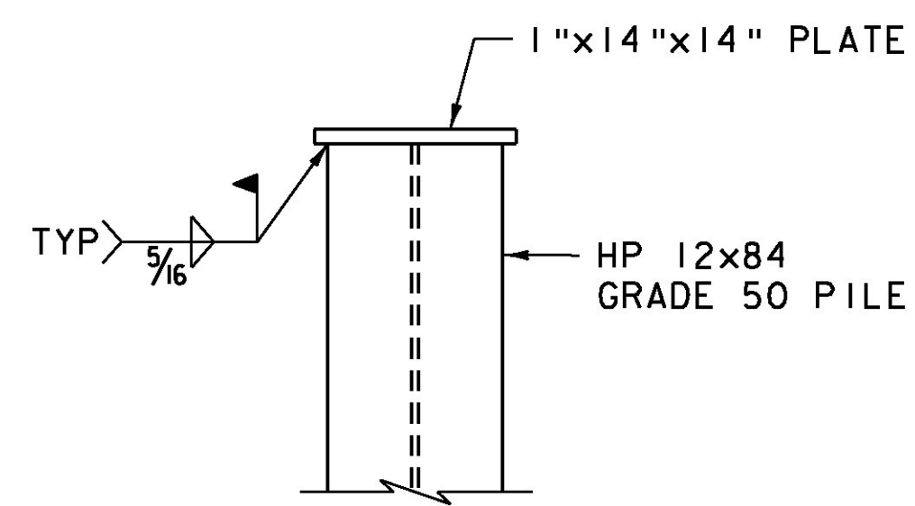
PILE PLATE SCALE 1" = 1'-0"
