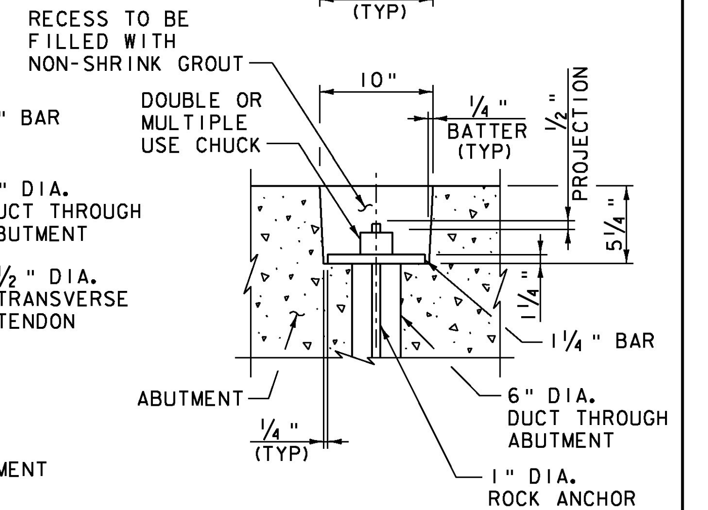
ROCK ANCHOR DETAIL NOT TO SCALE
