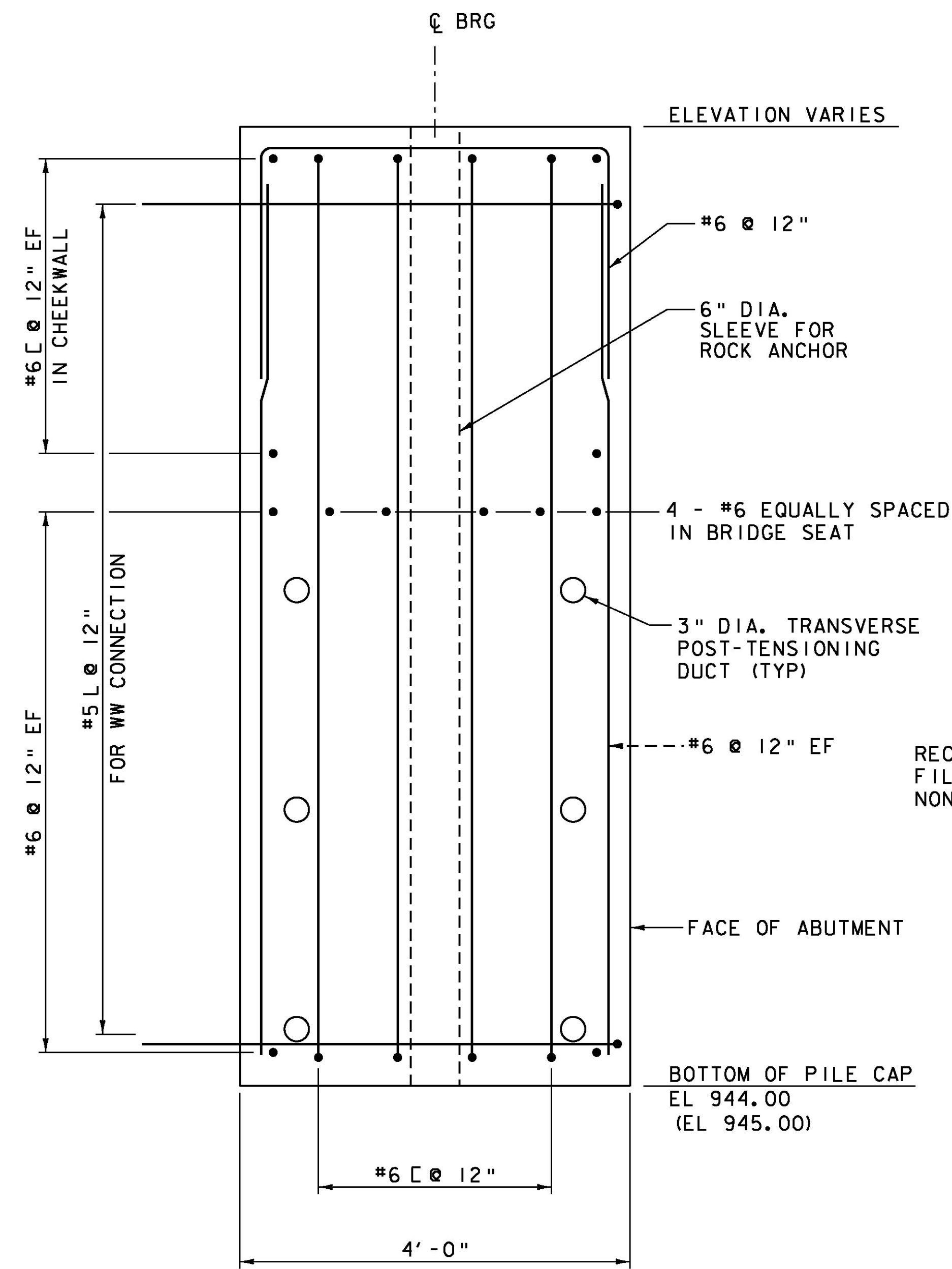
SECTION B-B SCALE 1" = 1'-0"
