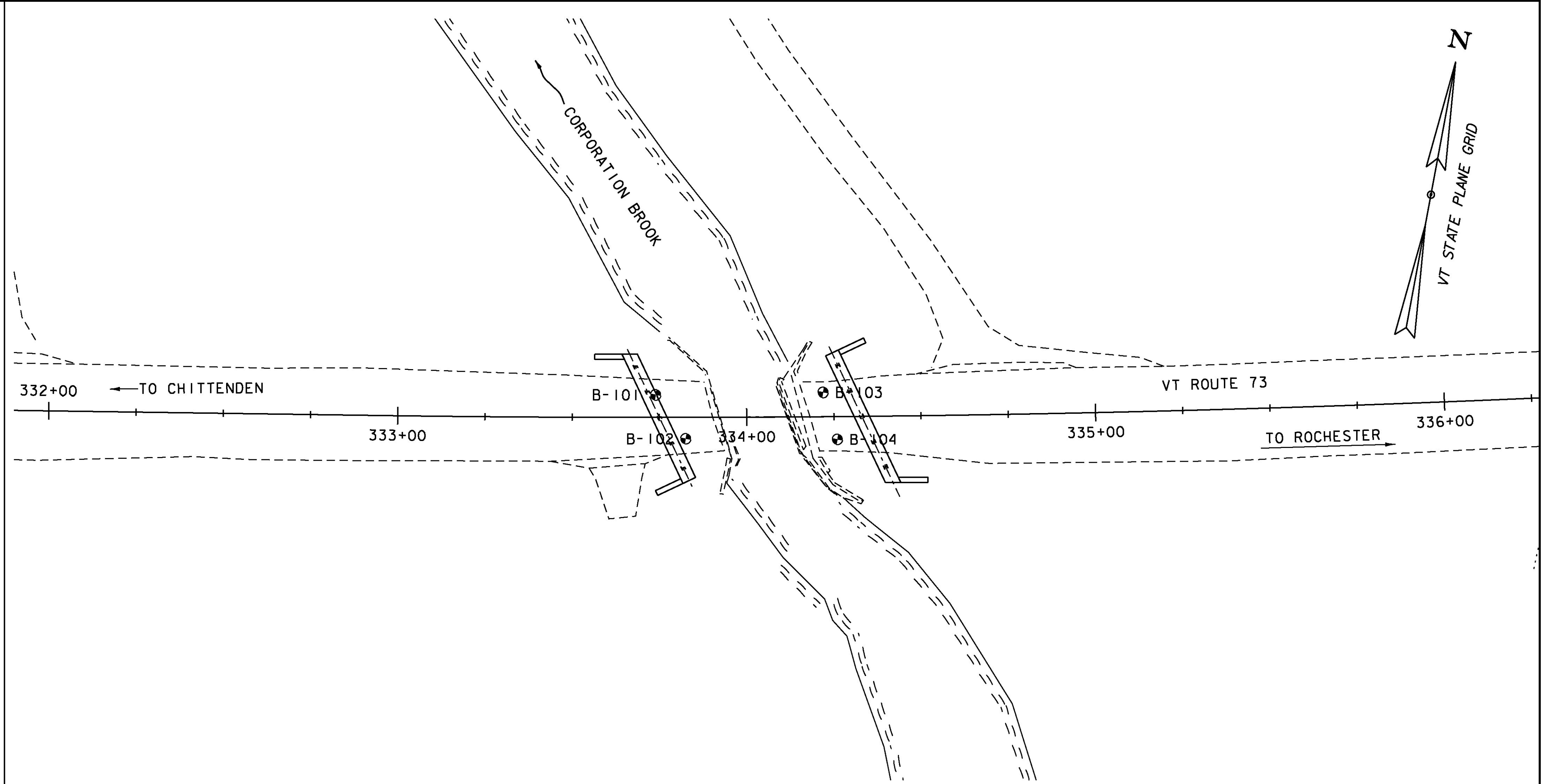
BORING LAYOUT
