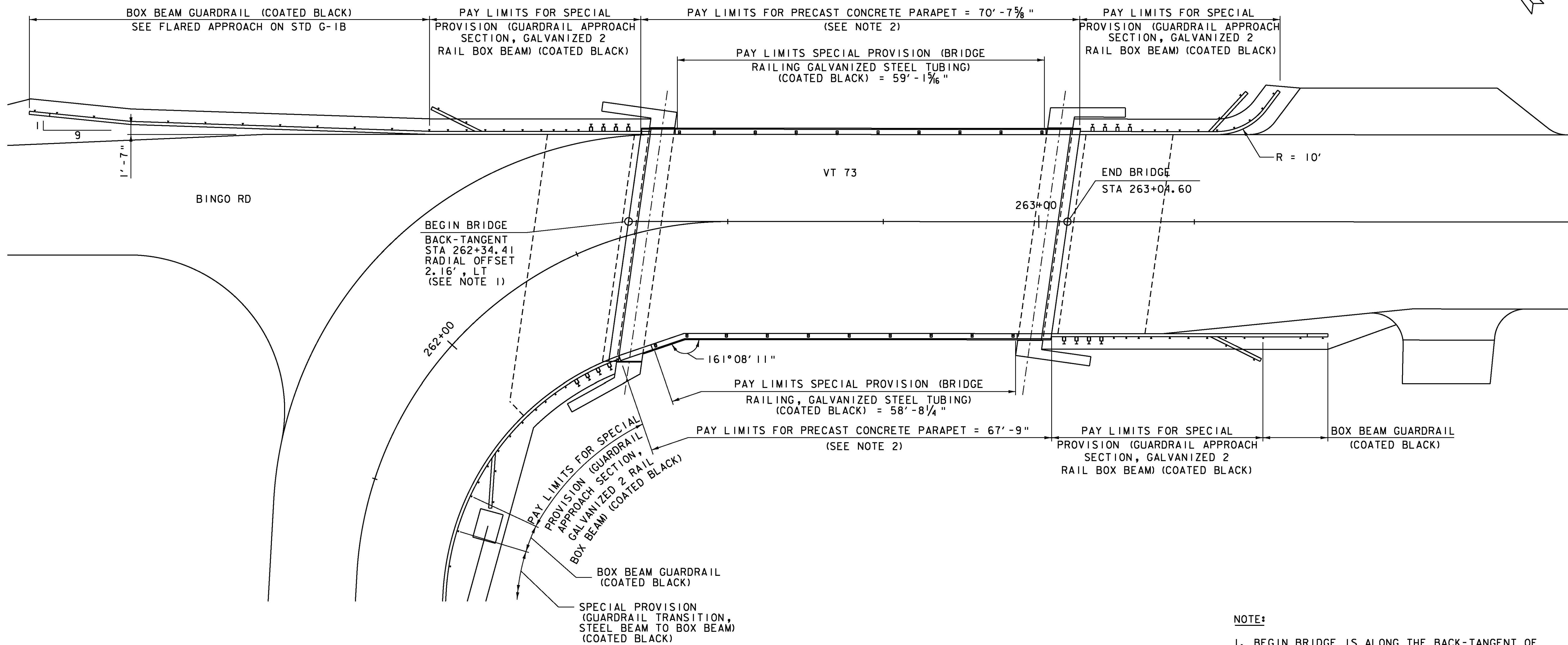
BRIDGE RAIL LAYOUT SCALE 1/8" = 1'-0"
