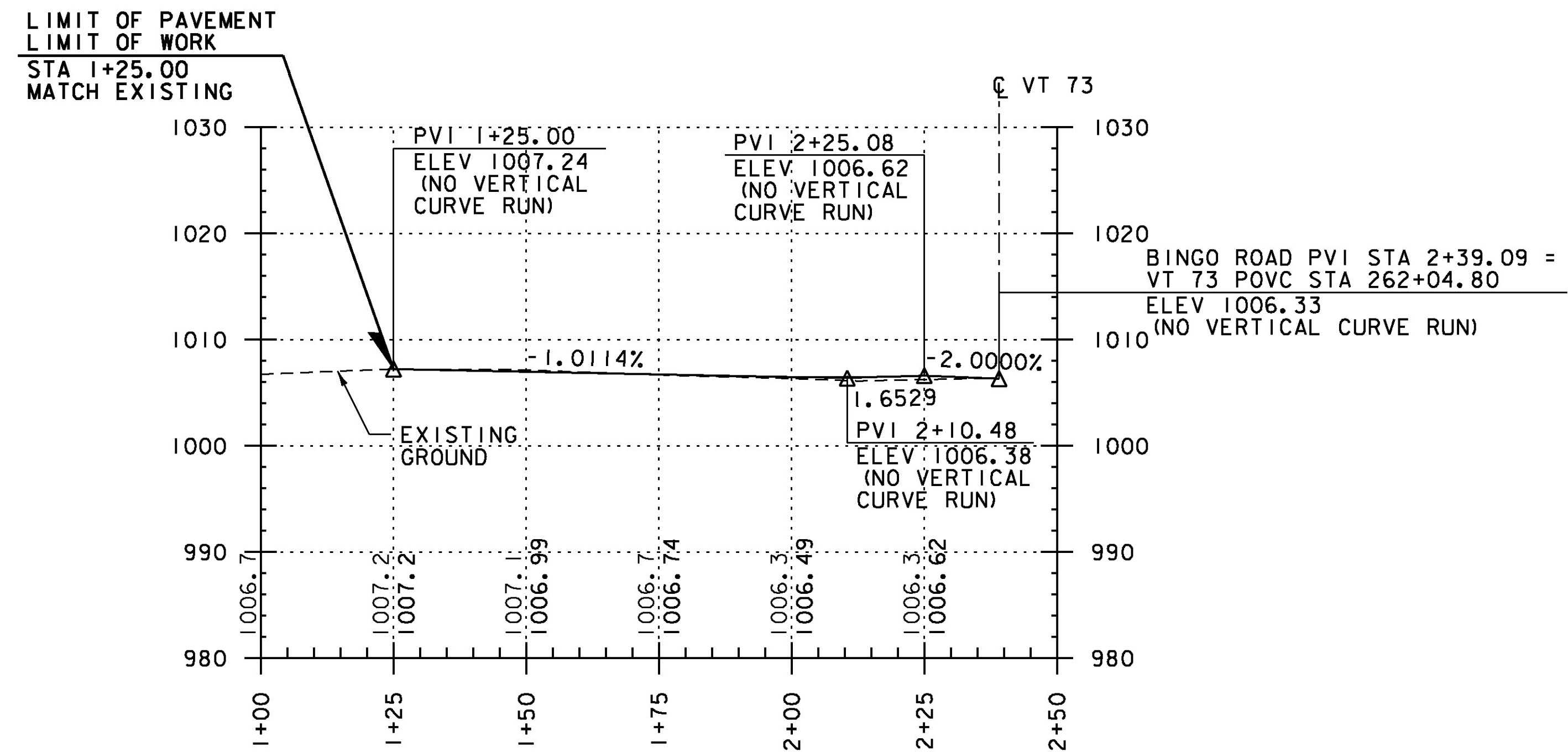
BINGO ROAD PROFILE SCALE 1" = 20' HORIZONTAL 1" = 10' VERTICAL
