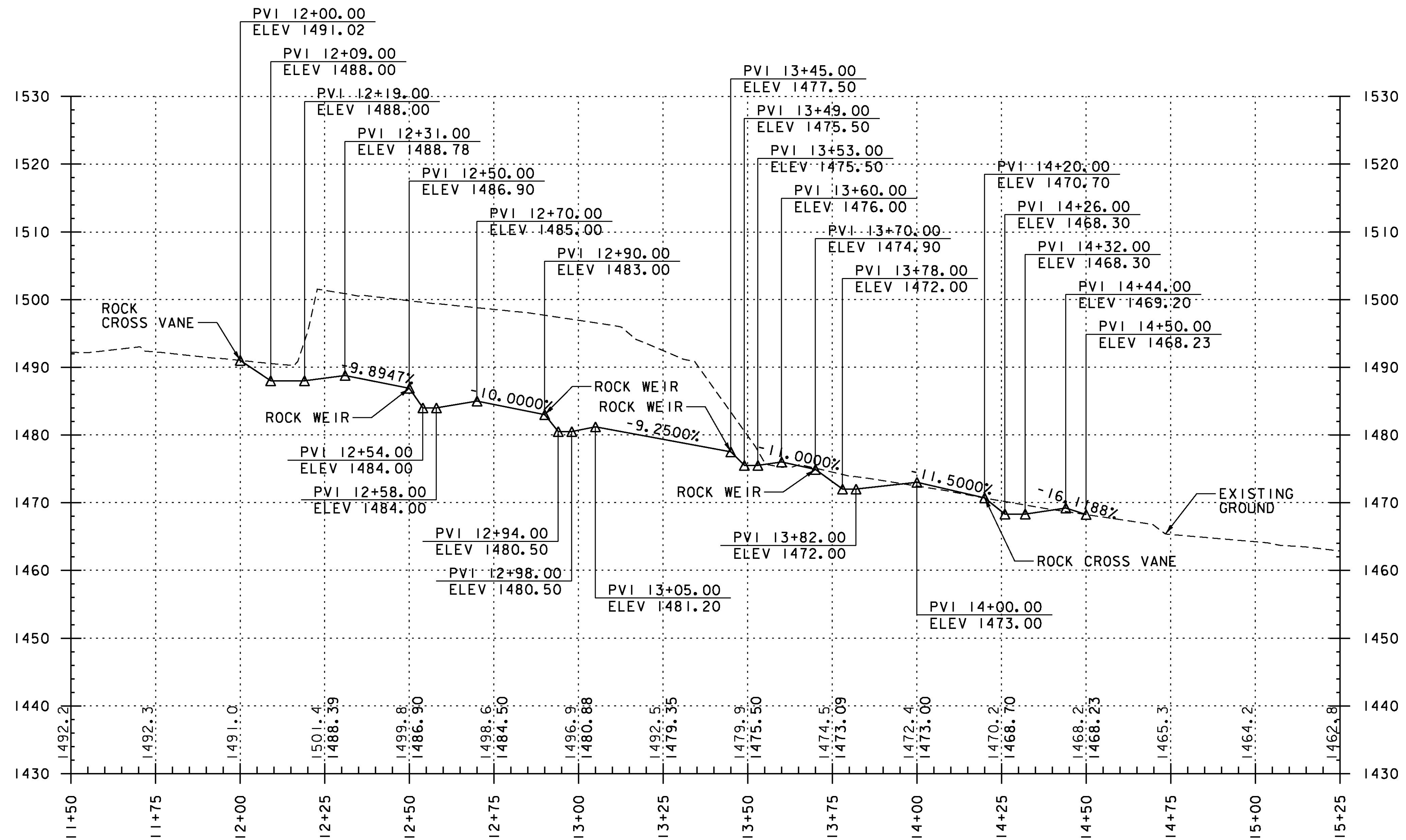
BRANDON BROOK PROFILE SCALE 1" = 20' HORIZONTAL 1" = 10' VERTICAL
