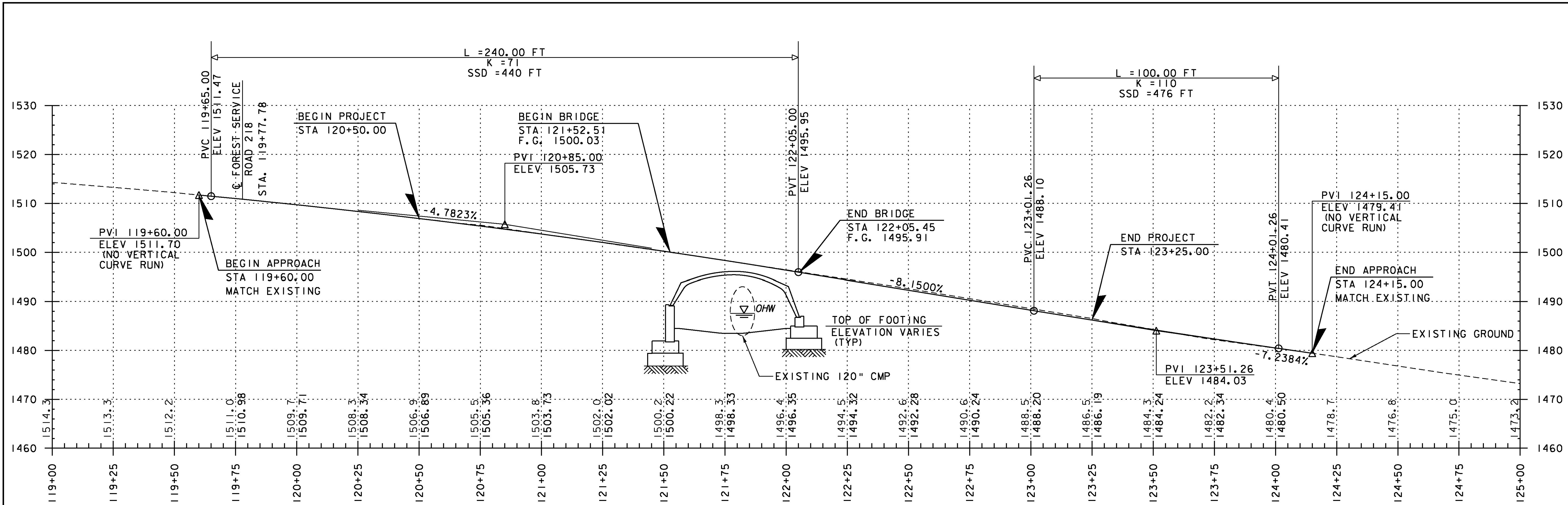
VT 73 PROFILE SCALE 1" = 20' HORIZONTAL 1" = 10' VERTICAL
