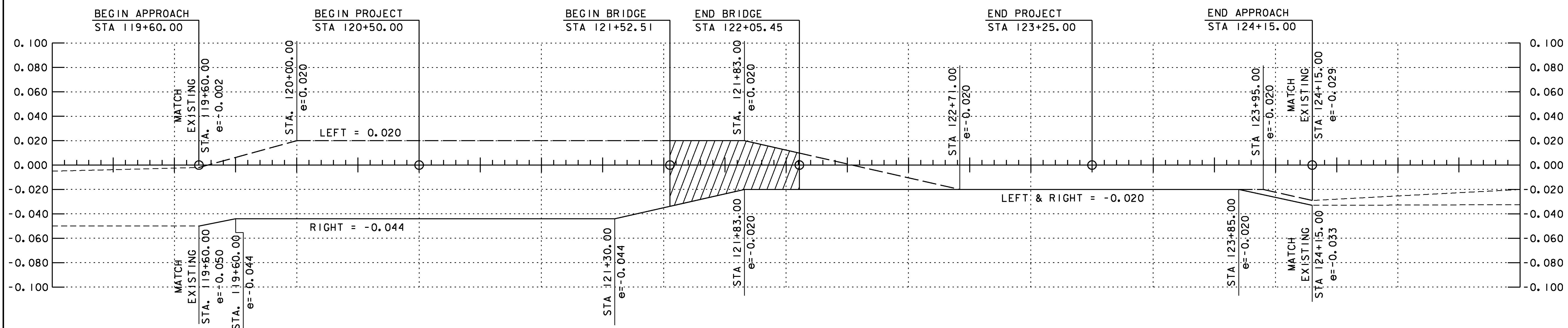
VT 73 BANKING DIAGRAM SCALE 1" = 20' HORIZONTAL 1" = 0.040 FT/FT VERTICAL
