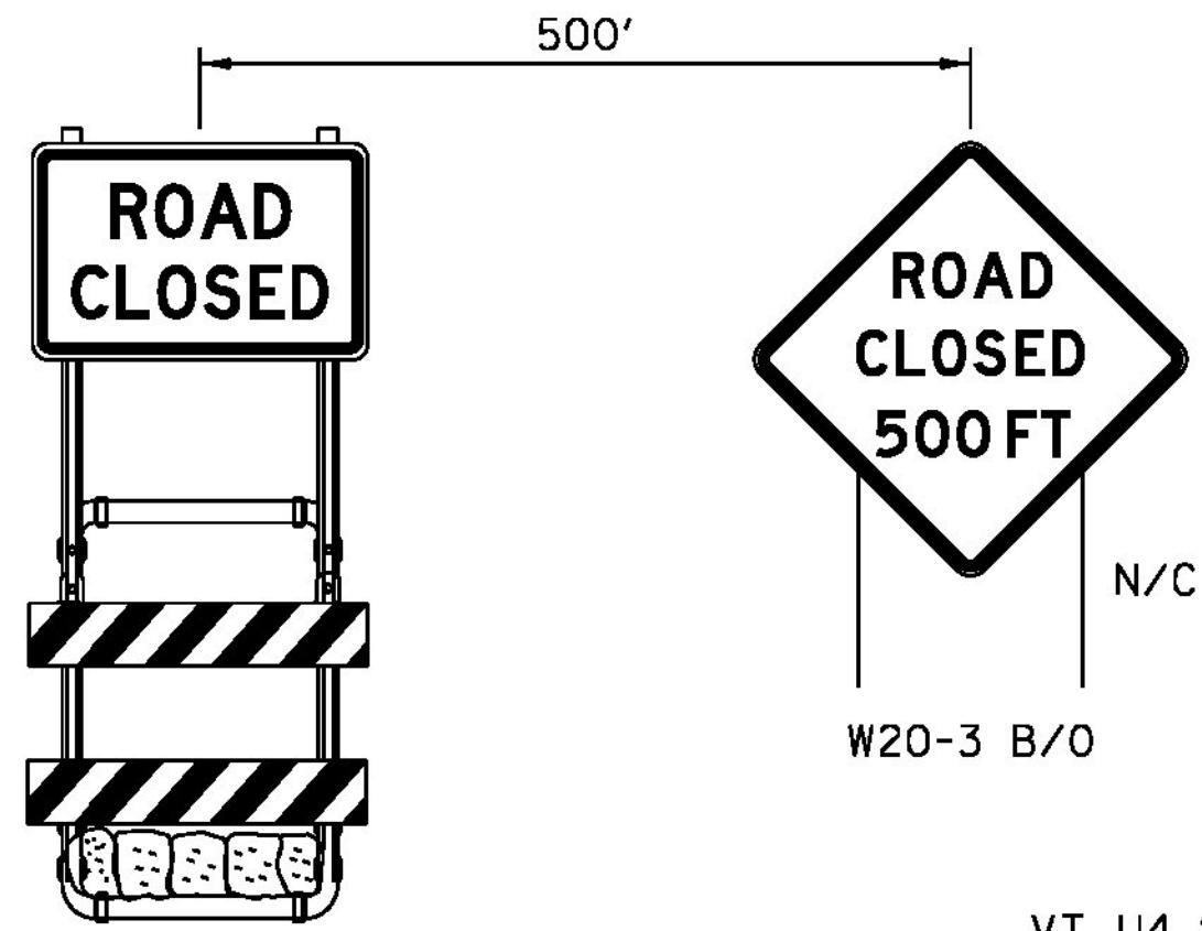
R11-2 B/W SIGN MOUNTED ON TYPE III BARRICADE (MODIFIED)
