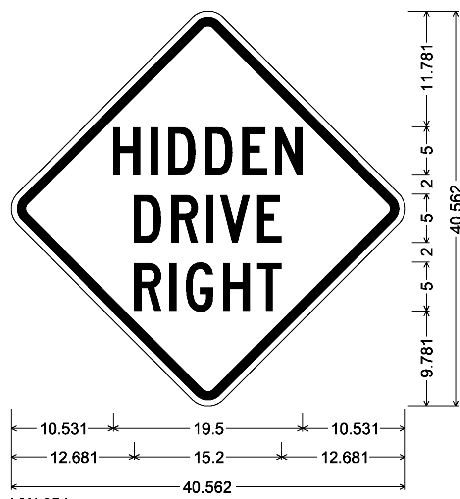
VW-054; 30.000" across sides 2.250" Radius, 0.875" Border, 0.625" Indent, Black on Yellow; [HIDDEN] C 2K; [DRIVE] C 2K; [RIGHT] C 2K;
