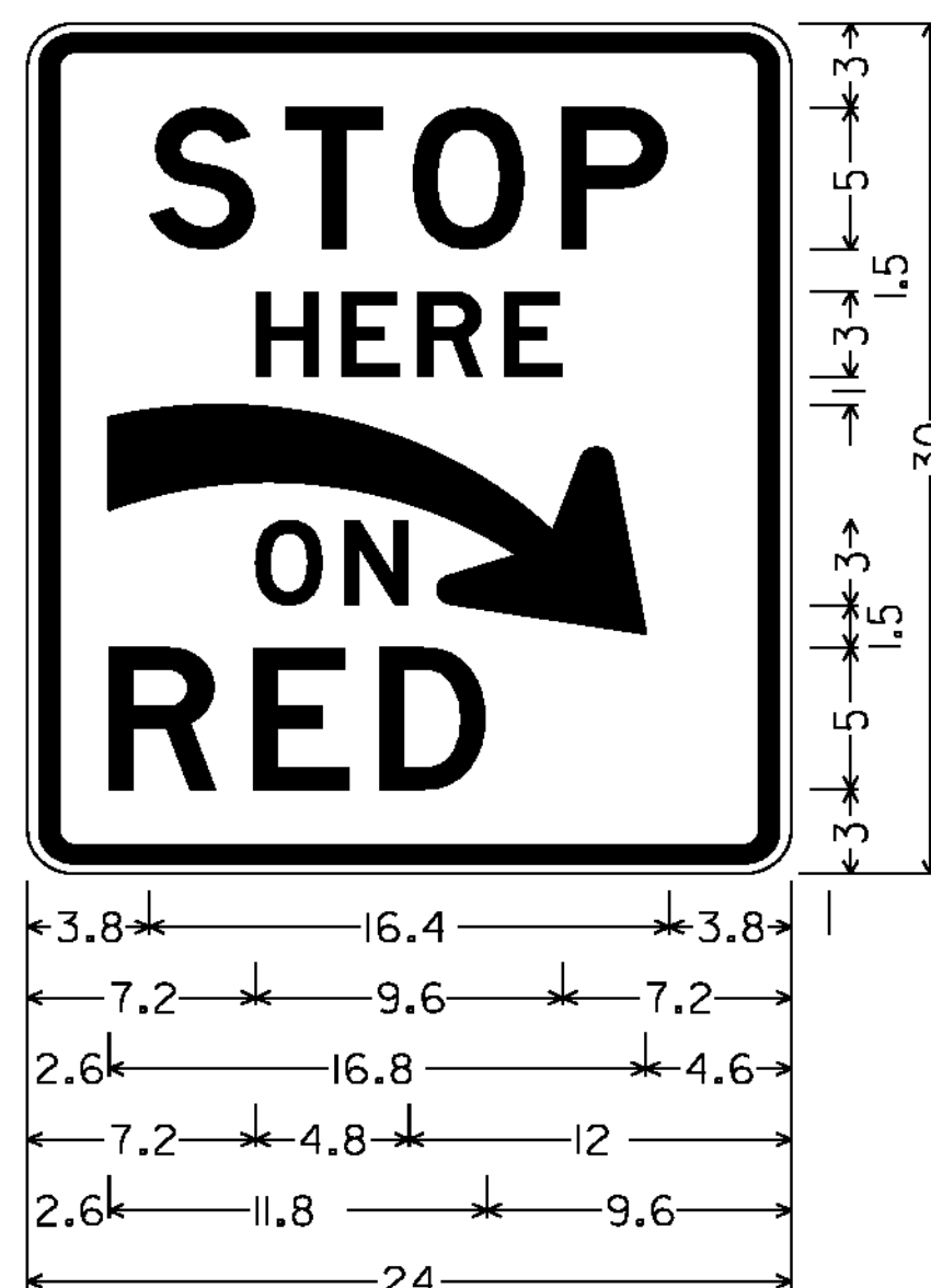
1.500" RADIUS, 0.625" BORDER, 0.375" INDENT, BLACK ON WHITE; [STOP] 5"D; [HERE] 3"D; [ON] 3"D; [RED] 5"D RIO-6aRM
