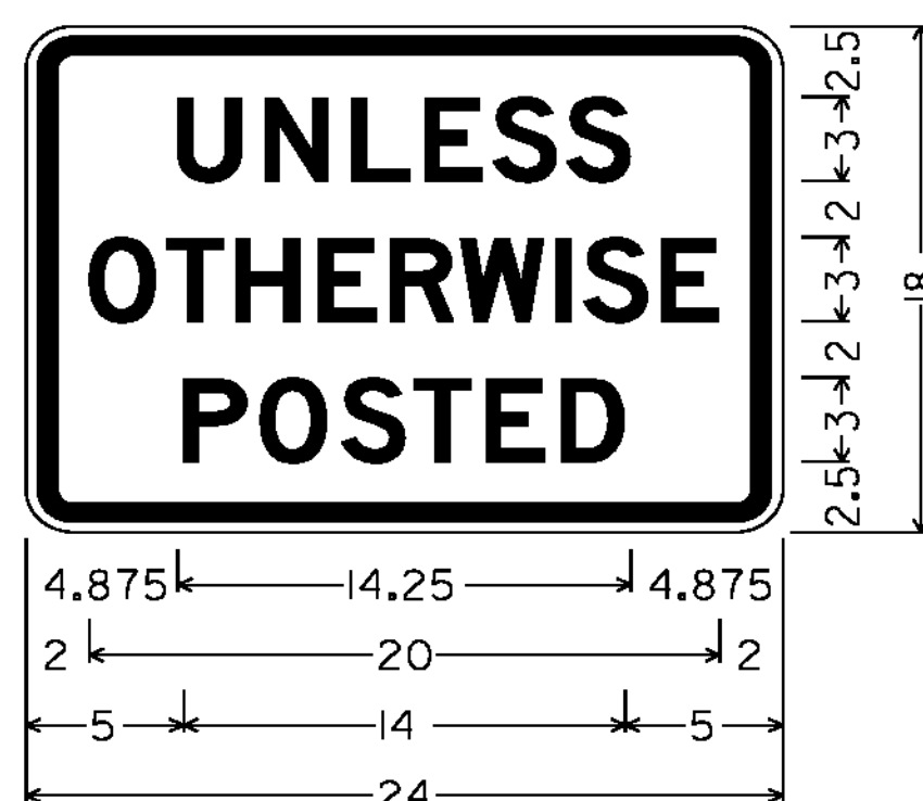
1.500" RADIUS, 0.625" BORDER, 0.375" INDENT, BLACK ON WHITE; [UNLESS] 2"D; [OTHERWISE] 2"D; [POSTED] 2"D R2-5P
