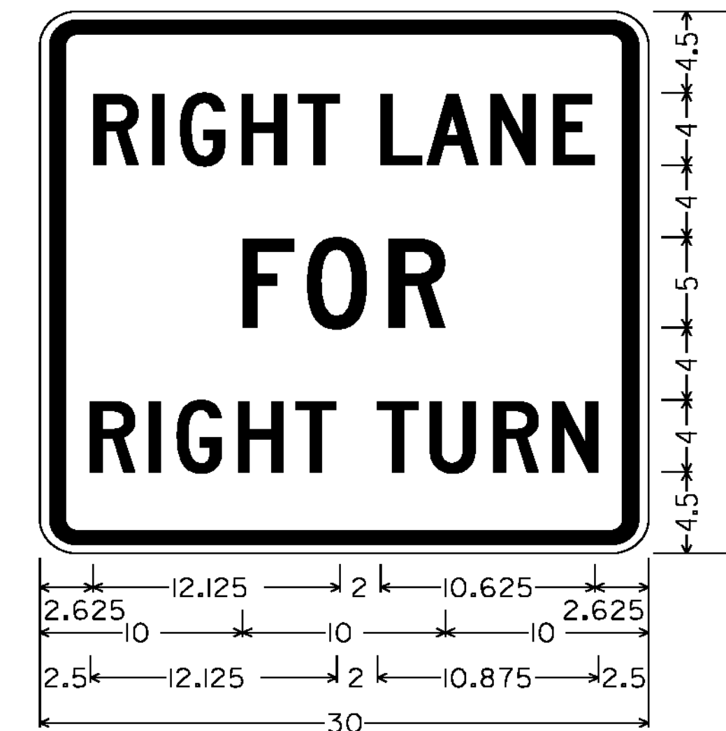
1.875" RADIUS, 0.750" BORDER, 0.500" INDENT, BLACK ON WHITE; [RIGHT LANE] 2"C; [FOR] 2"C; [RIGHT TURN] 2"C VR-127
