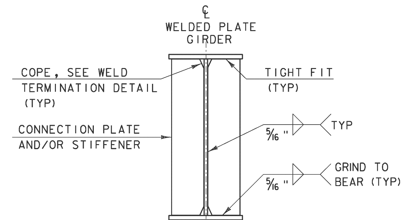
PIER BEARING STIFFENERS AND/OR CONNECTION PLATES FOR WELDED PLATE GIRDERS
