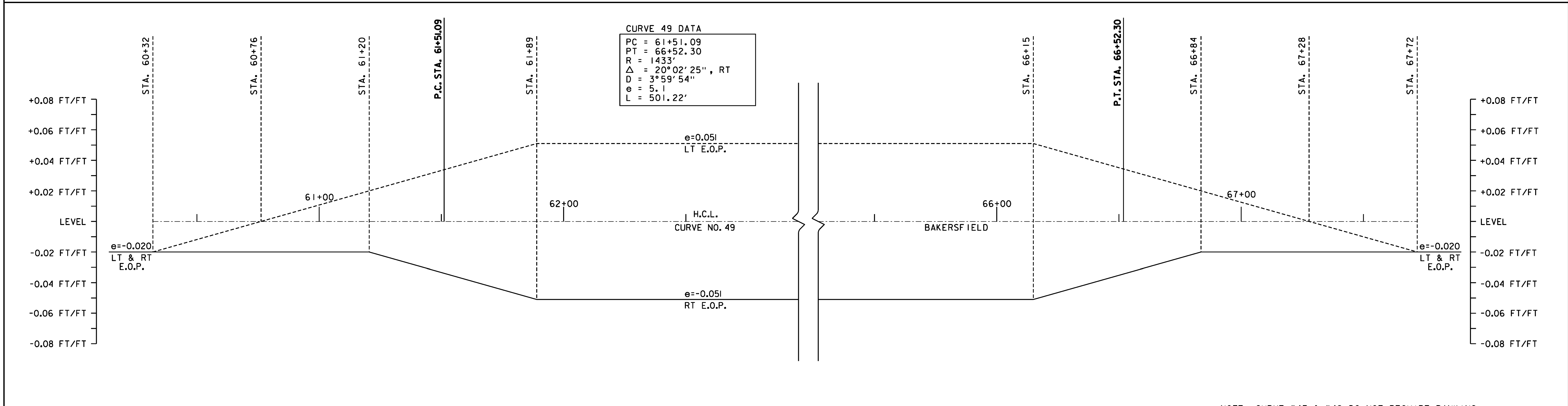
CURVE 45 & 46 BANKING TRANSITION DIAGRAM
