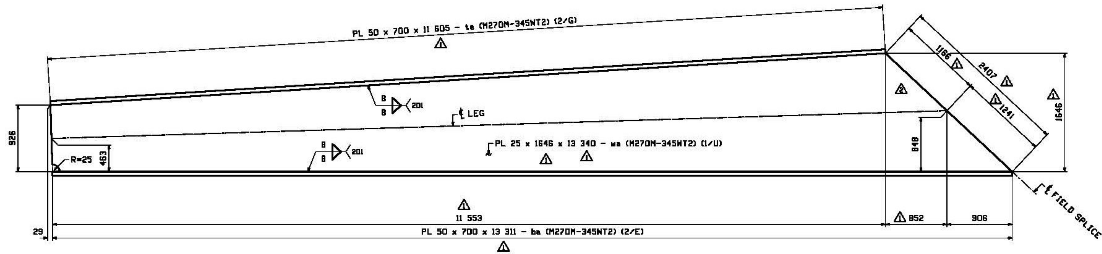
WEB AND FLANGE CUTTING DIAGRAMS FOR GIRDERS 21L1S, 22L2S, 23L3S, 24L4S, 25L5S, 21L5N, 22L4N, 23L3N, 24L2N & 25L1N
