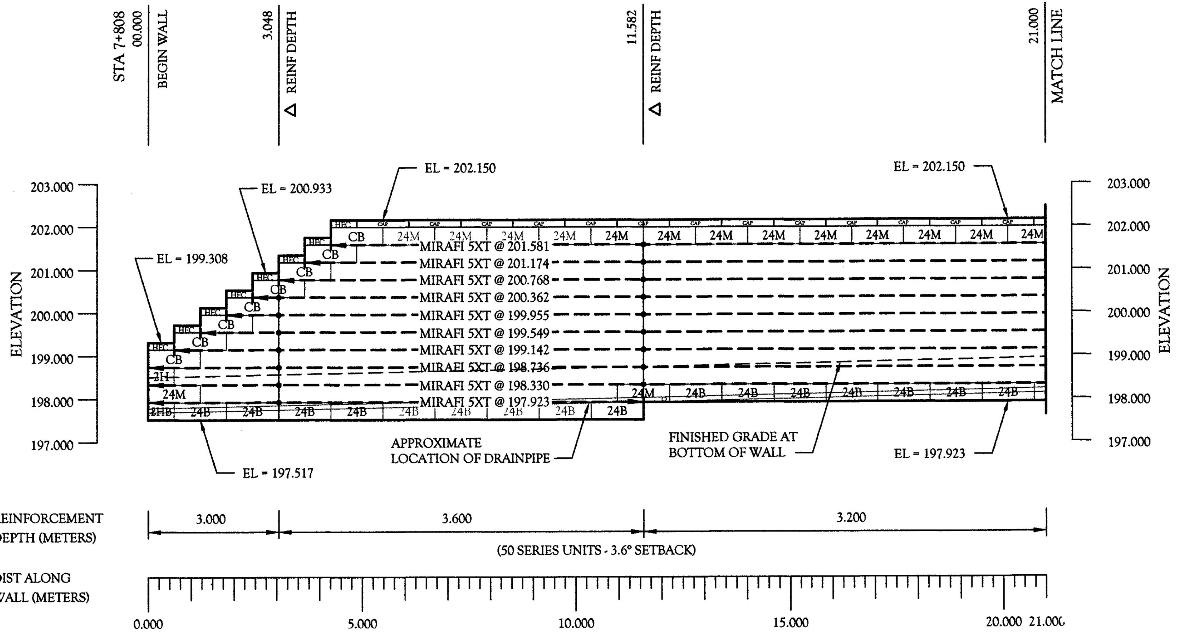
RECON WALL 1 - FRONT FACE ELEVATION
