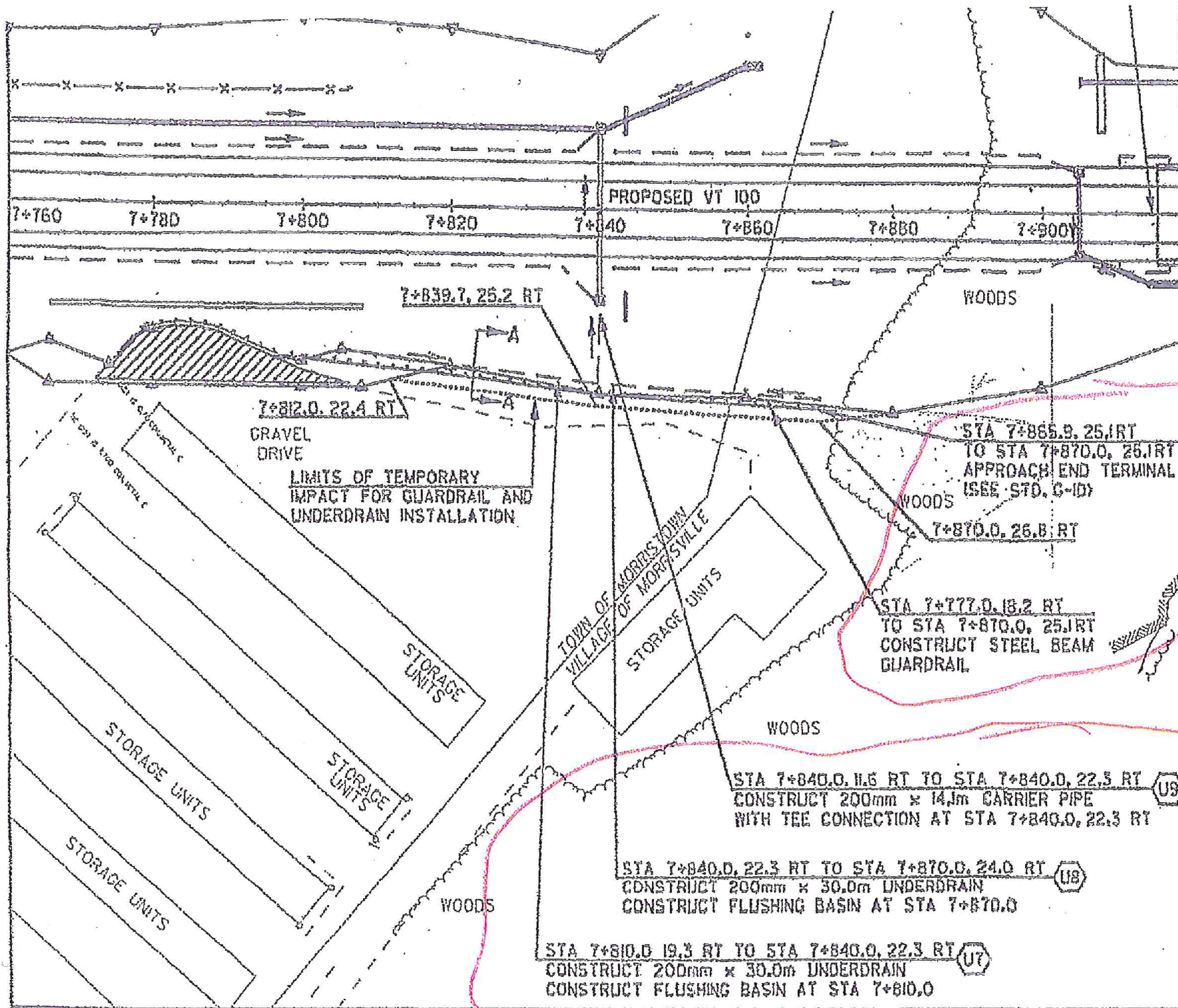
PLAN VIEW
