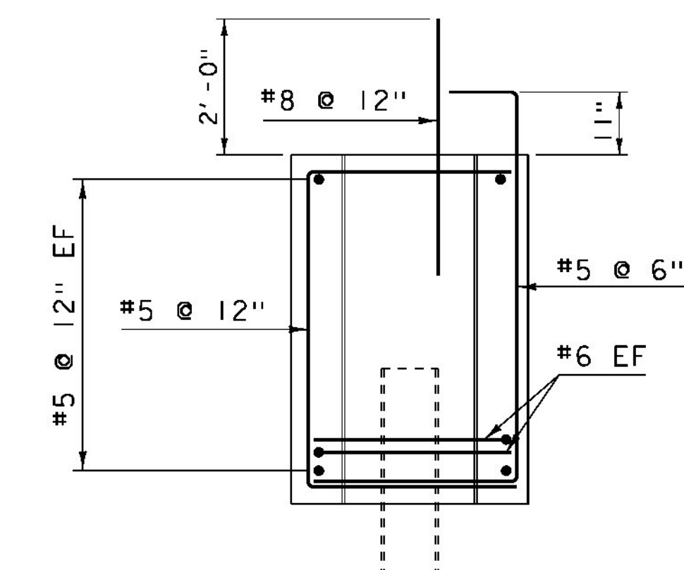
SECTION B-B
