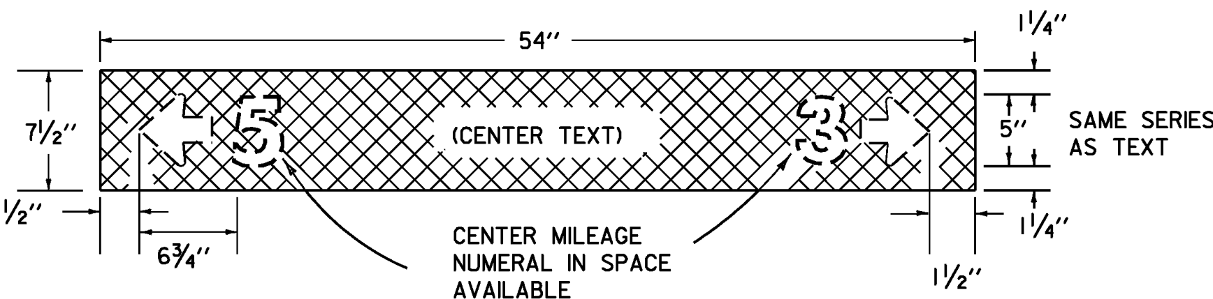
SIGN & LEGEND LAYOUT DIMENSIONS
