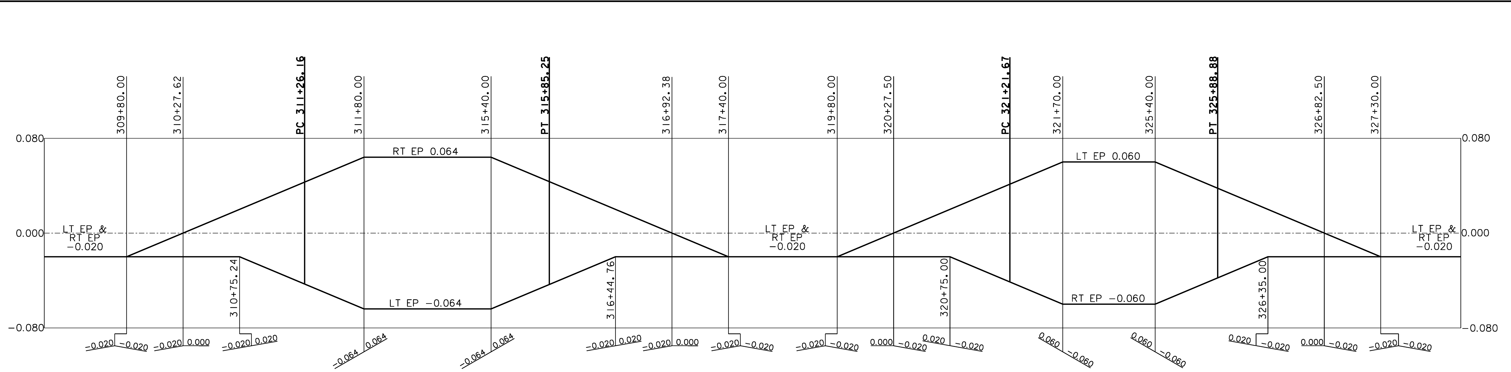
CURVE 25 - WEATHERSFIELD
