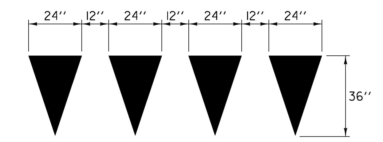
YIELD LINE DETAILS
