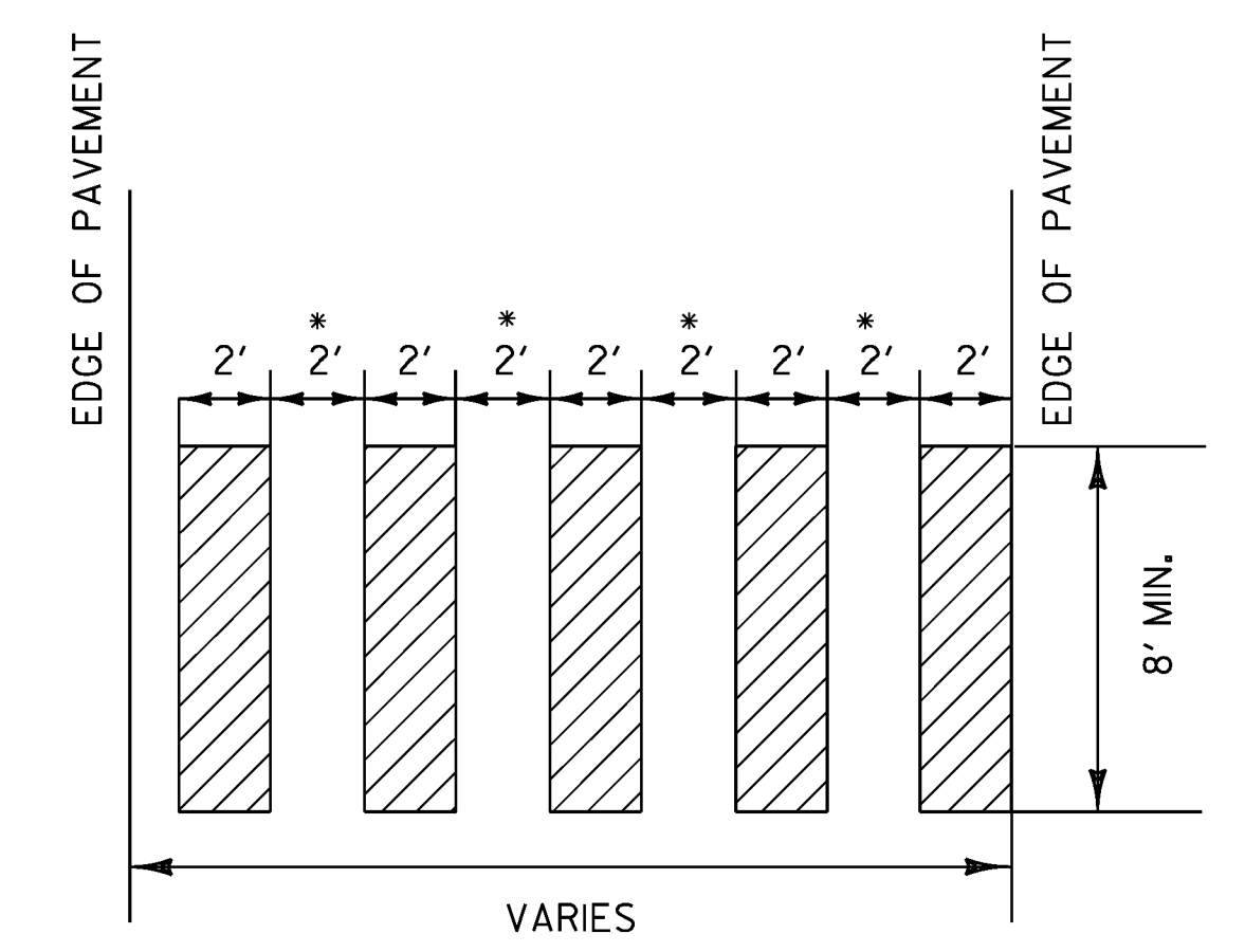
BLOCK PATTERN CROSSWALK DETAIL
