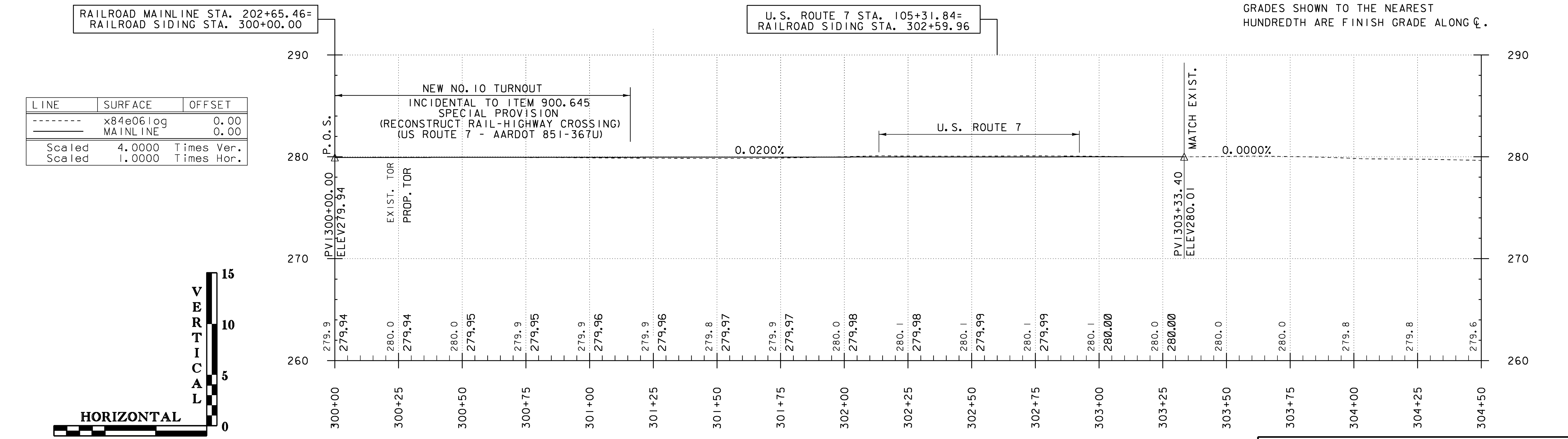
RAILROAD SIDING TOP OF RAIL PROFILE
