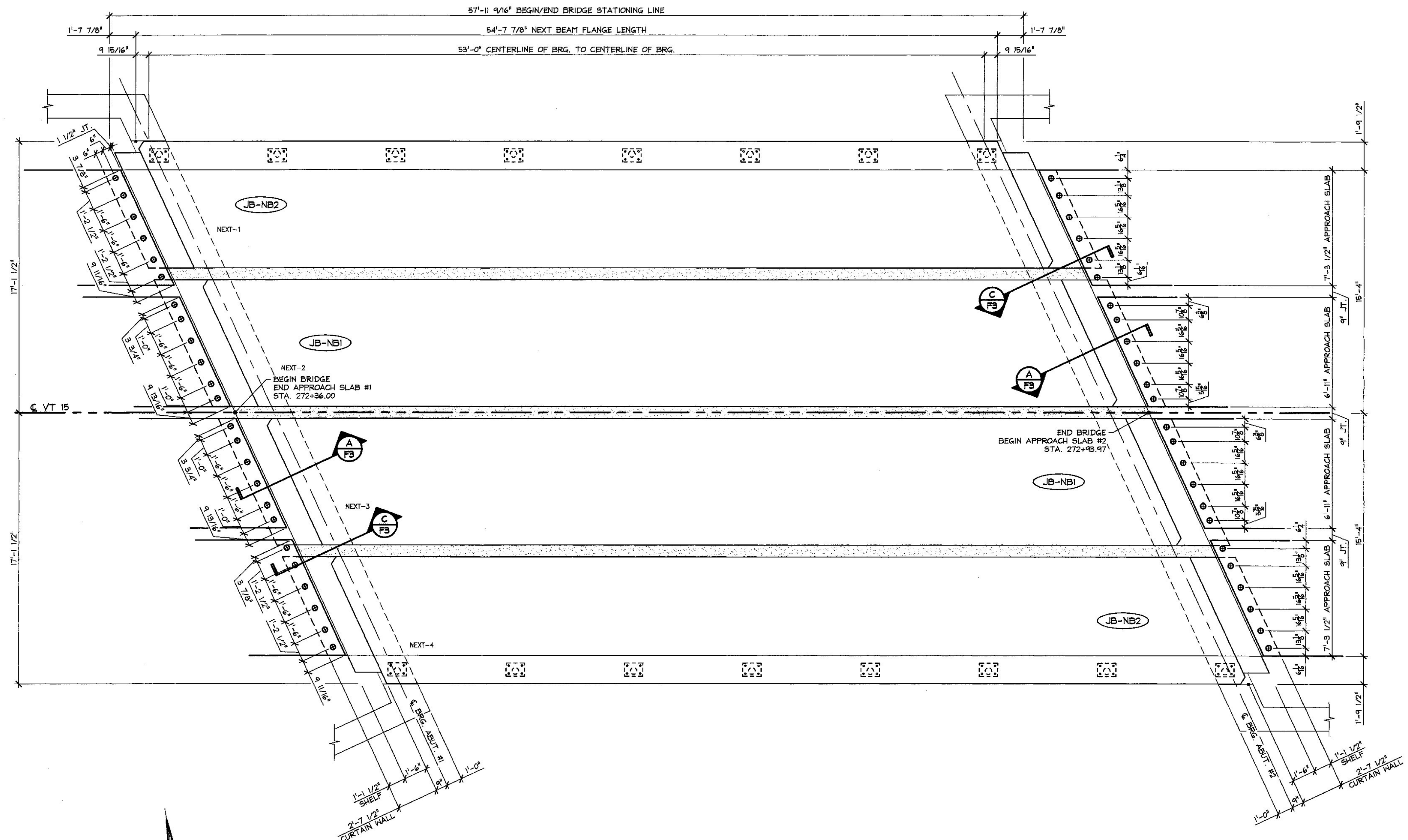
1 APPROACH SLAB ANCHOR DOWEL LOCATION PLAN F1.1 1/4" = 1'-0"
