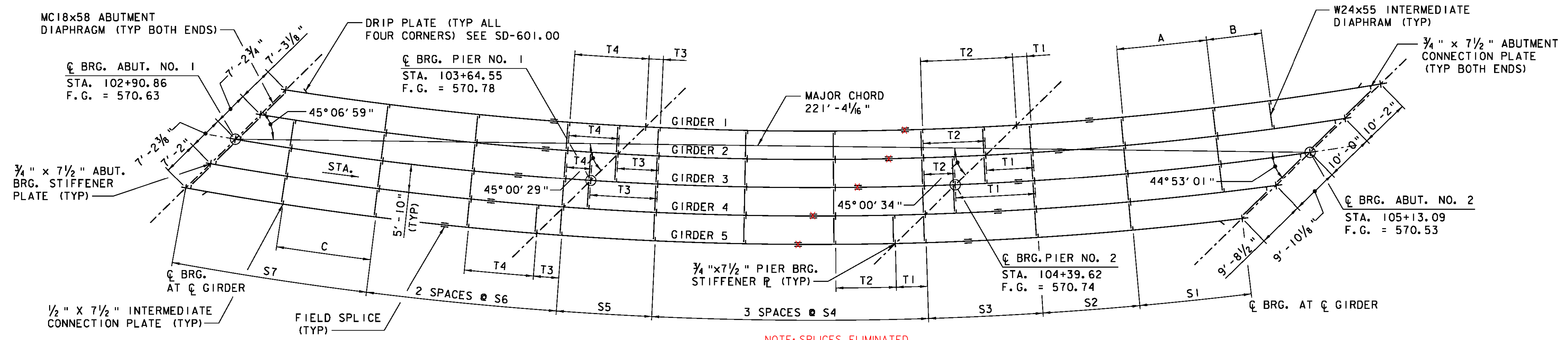
FRAMING PLAN SCALE 1/2" = 1'-0"
