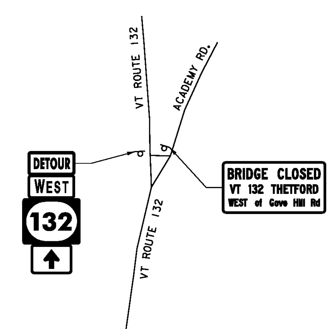
DETAIL J NOT TO SCALE
