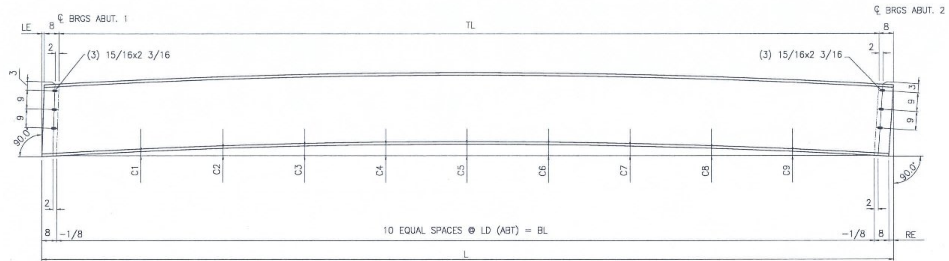
CAMBER DIAGRAM
