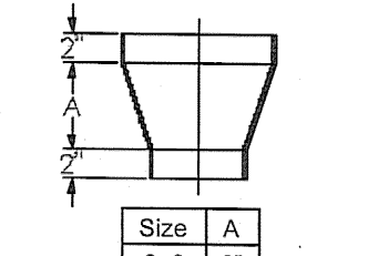
Drain Reducer
