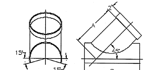
45° Lateral Saddle
