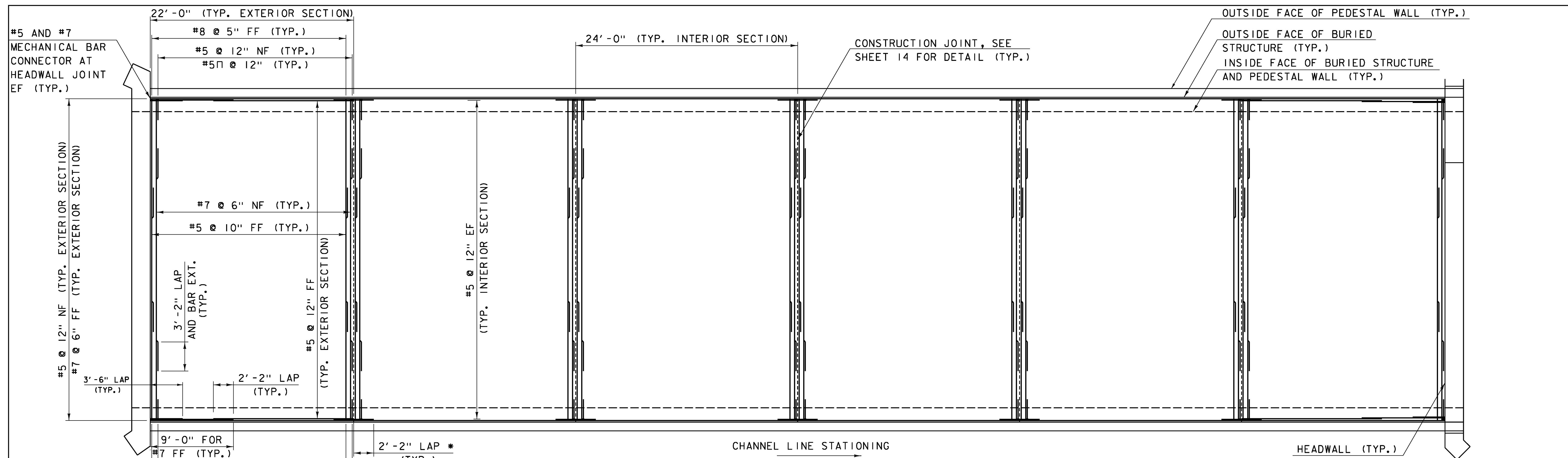
US 5 BURIED STRUCTURE REINFORCING - PLAN
