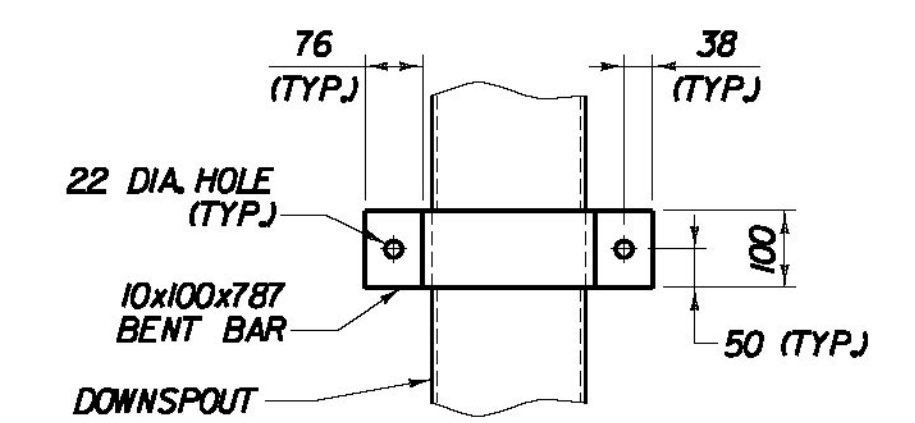
MOUNTING BRACKET ELEVATION SCALE 1/10
