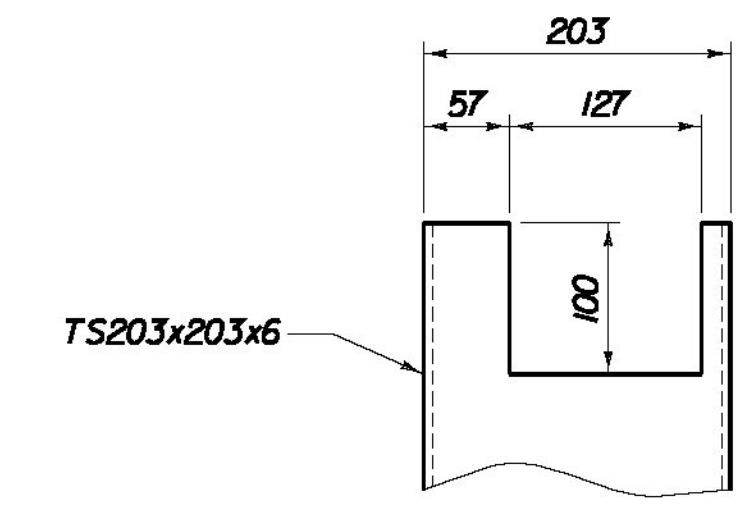
DOWNSPOUT CUTOUT FOR TROUGH SCALE 1/5
