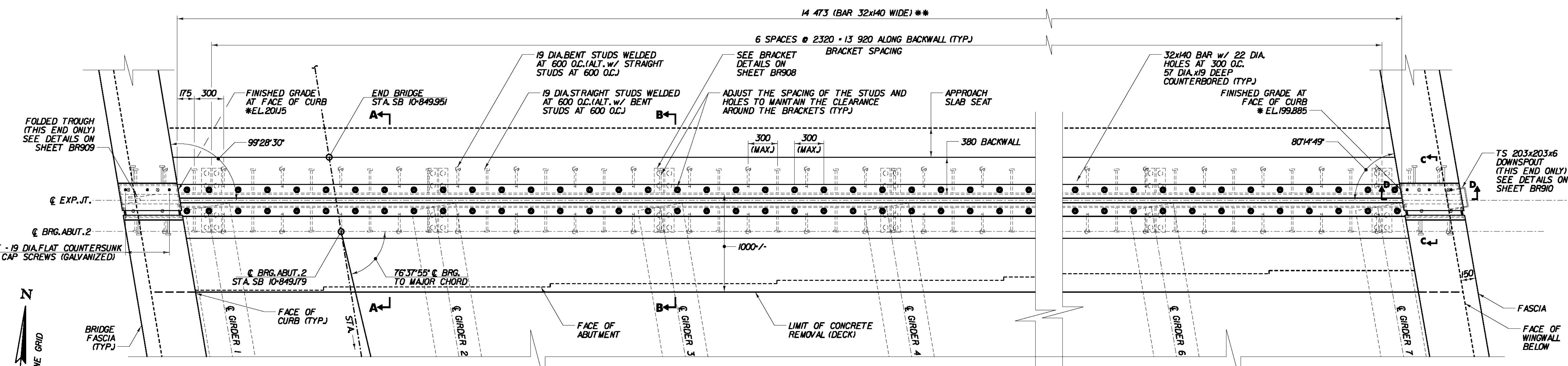
ABUTMENT 2 EXPANSION JOINT PLAN SCALE 1:20
