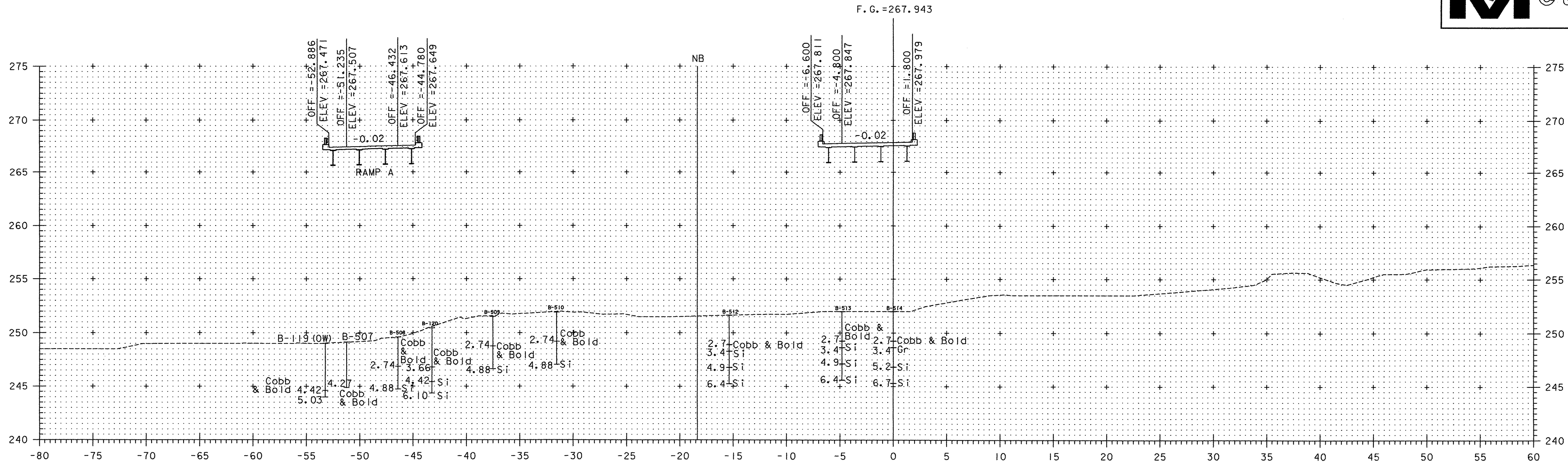
D 1+340.000 = A 1+334.865
