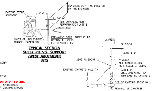
TYPICAL SECTION @ WEST ABUTMENT 3/4" = 1'-0"
