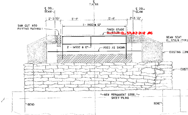
ELEVATION WEST ABUTMENT 1/2" = 1'-0"
